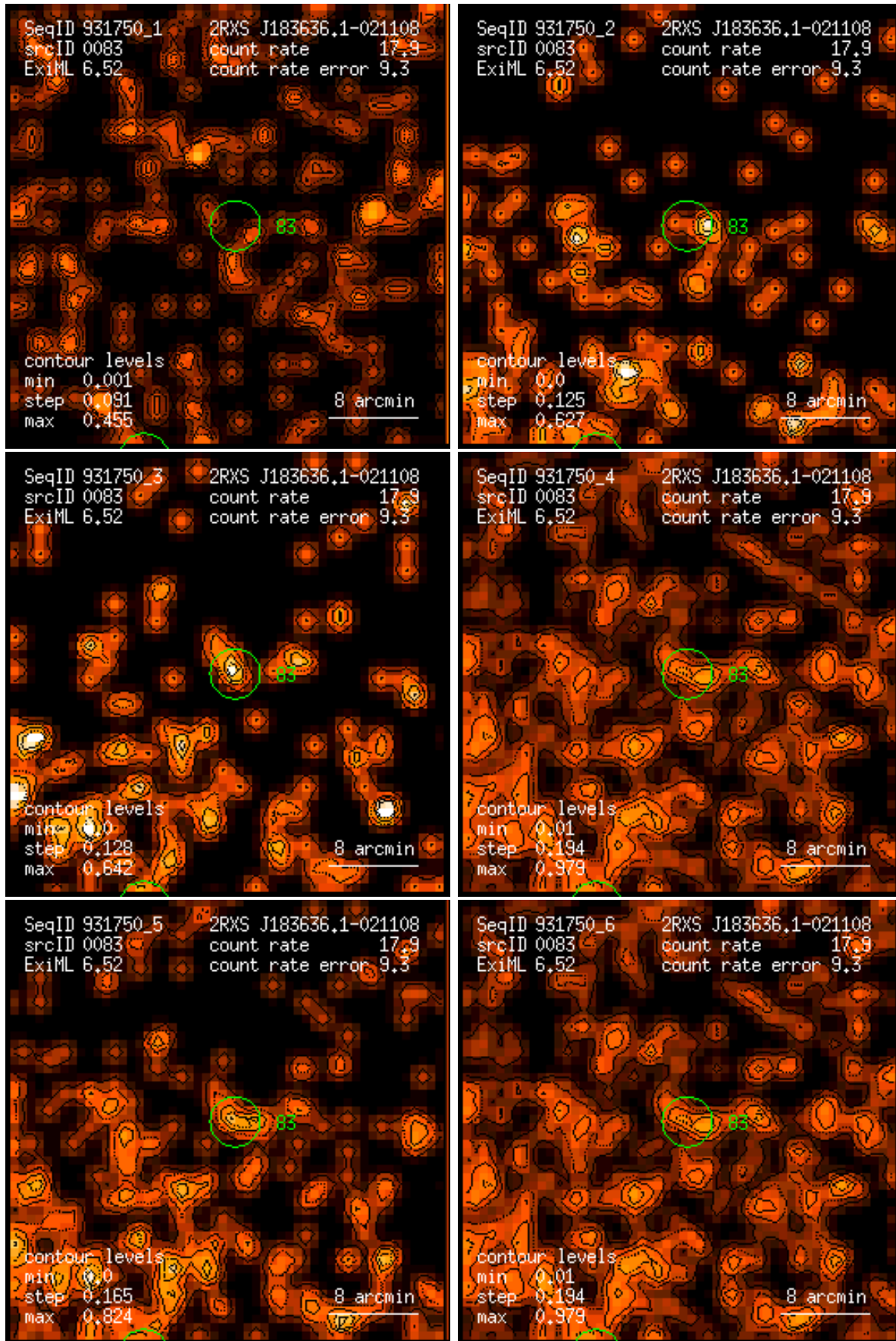
Figure 83: RASS 931750: detection 0083: band rate images, Gaussian filter: (1) PSPC channels 11 – 41, (2) 52 – 90, (3) 91 – 201, (4) 11 – 235, (5) 52 – 201, (6) 11 – 201. Broad band rates in counts/ks. Band rate contour levels in counts/ks/arcmin 2 .
