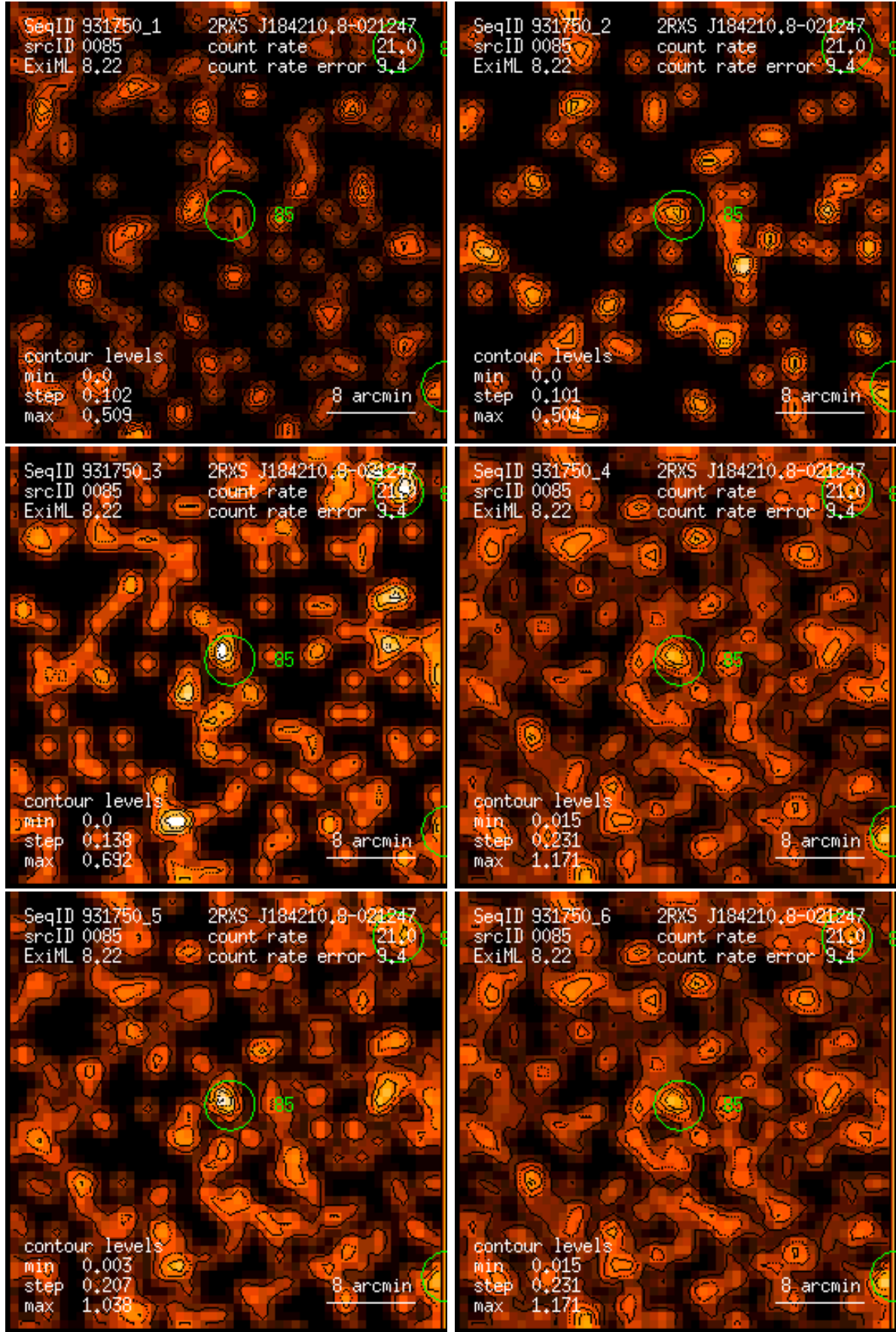
Figure 85: RASS 931750: detection 0085: band rate images, Gaussian filter: (1) PSPC channels 11 – 41, (2) 52 – 90, (3) 91 – 201, (4) 11 – 235, (5) 52 – 201, (6) 11 – 201. Broad band rates in counts/ks. Band rate contour levels in counts/ks/arcmin 2 .
