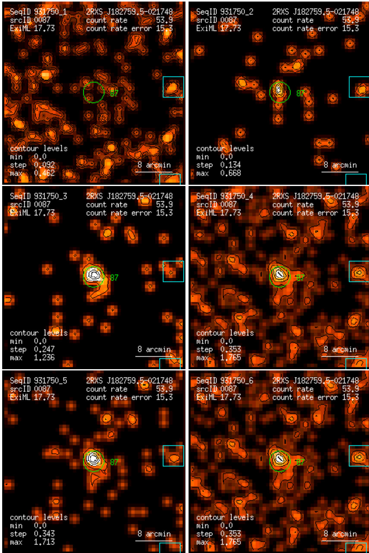
Figure 87: RASS 931750: detection 0087: band rate images, Gaussian filter: (1) PSPC channels 11 – 41, (2) 52 – 90, (3) 91 – 201, (4) 11 – 235, (5) 52 – 201, (6) 11 – 201. Broad band rates in counts/ks. Band rate contour levels in counts/ks/arcmin 2 .
