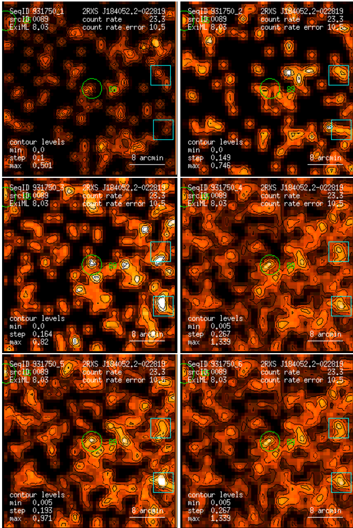
Figure 89: RASS 931750: detection 0089: band rate images, Gaussian filter: (1) PSPC channels 11 – 41, (2) 52 – 90, (3) 91 – 201, (4) 11 – 235, (5) 52 – 201, (6) 11 – 201. Broad band rates in counts/ks. Band rate contour levels in counts/ks/arcmin 2 .
