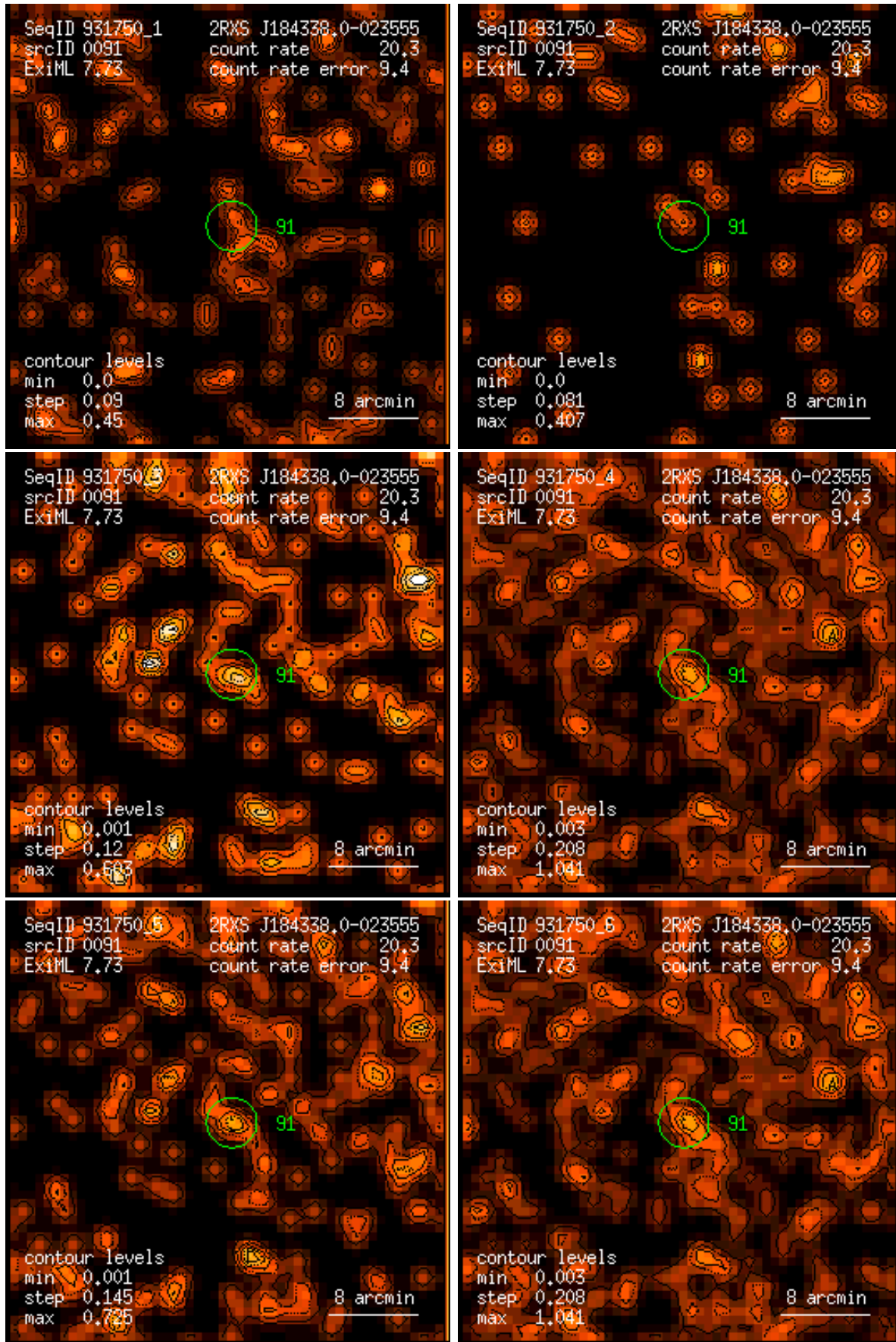
Figure 91: RASS 931750: detection 0091: band rate images, Gaussian filter: (1) PSPC channels 11 – 41, (2) 52 – 90, (3) 91 – 201, (4) 11 – 235, (5) 52 – 201, (6) 11 – 201. Broad band rates in counts/ks. Band rate contour levels in counts/ks/arcmin 2 .
