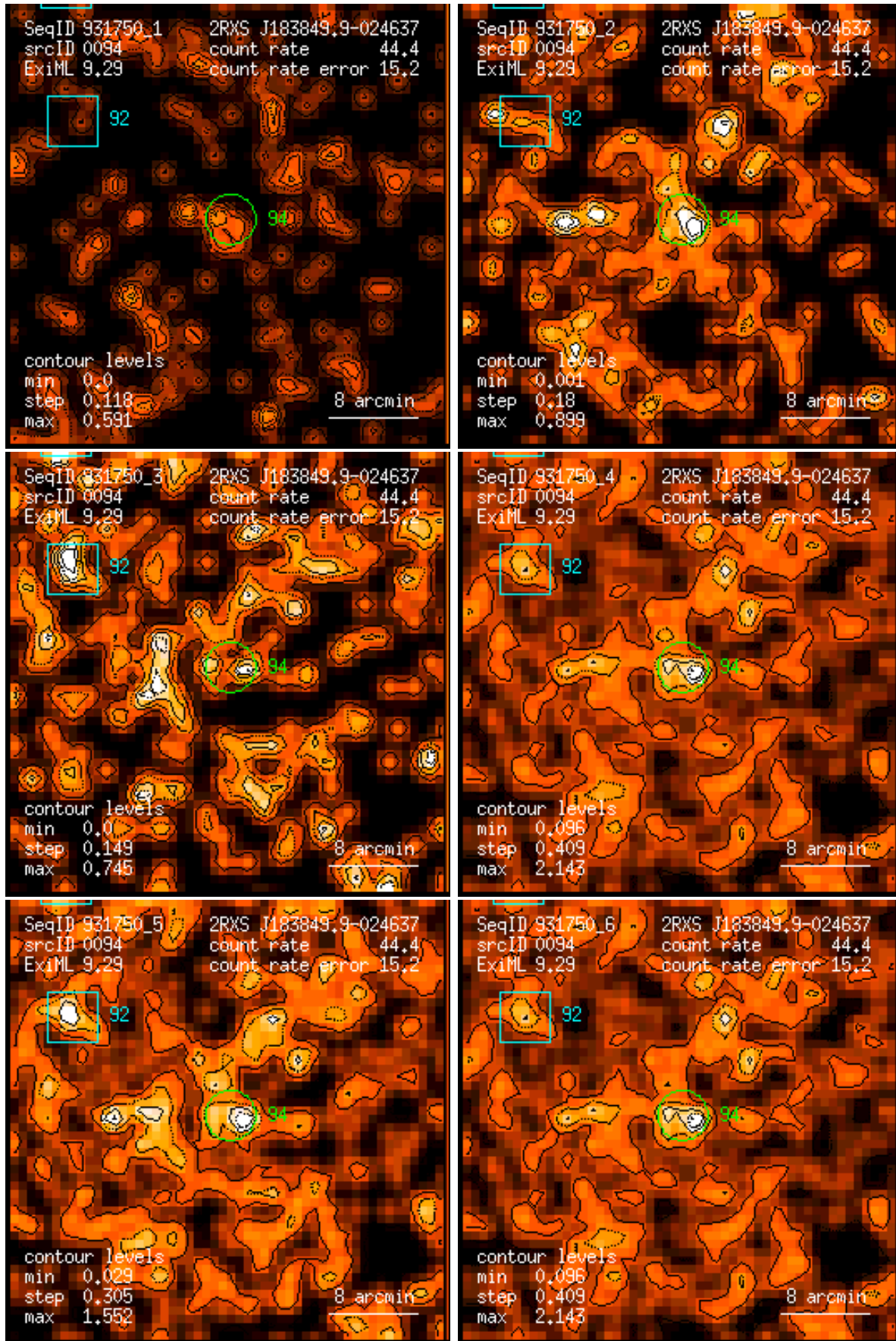
Figure 94: RASS 931750: detection 0094: band rate images, Gaussian filter: (1) PSPC channels 11 – 41, (2) 52 – 90, (3) 91 – 201, (4) 11 – 235, (5) 52 – 201, (6) 11 – 201. Broad band rates in counts/ks. Band rate contour levels in counts/ks/arcmin 2 .
