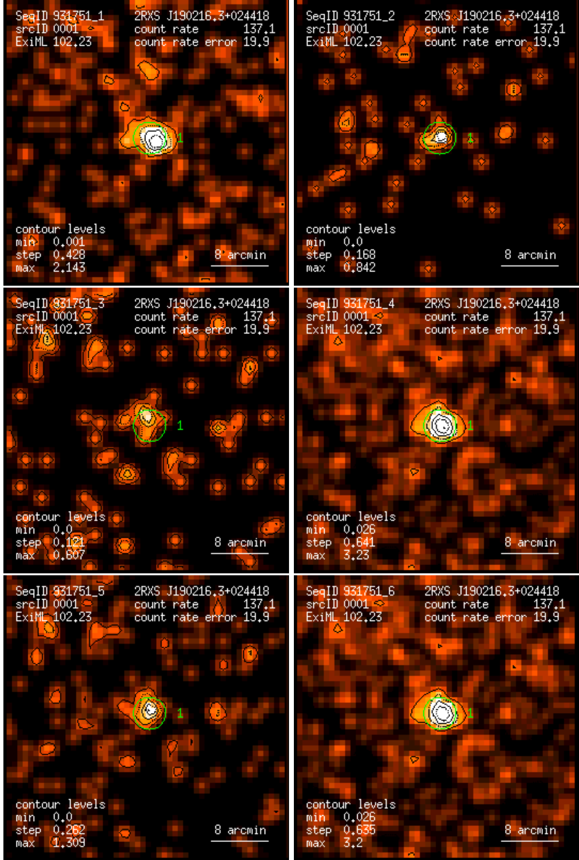
Figure 1: RASS 931751: detection 0001: band rate images, Gaussian filter: (1) PSPC channels 11 – 41, (2) 52 – 90, (3) 91 – 201, (4) 11 – 235, (5) 52 – 201, (6) 11 – 201. Broad band rates in counts/ks. Band rate contour levels in counts/ks/arcmin 2 .
