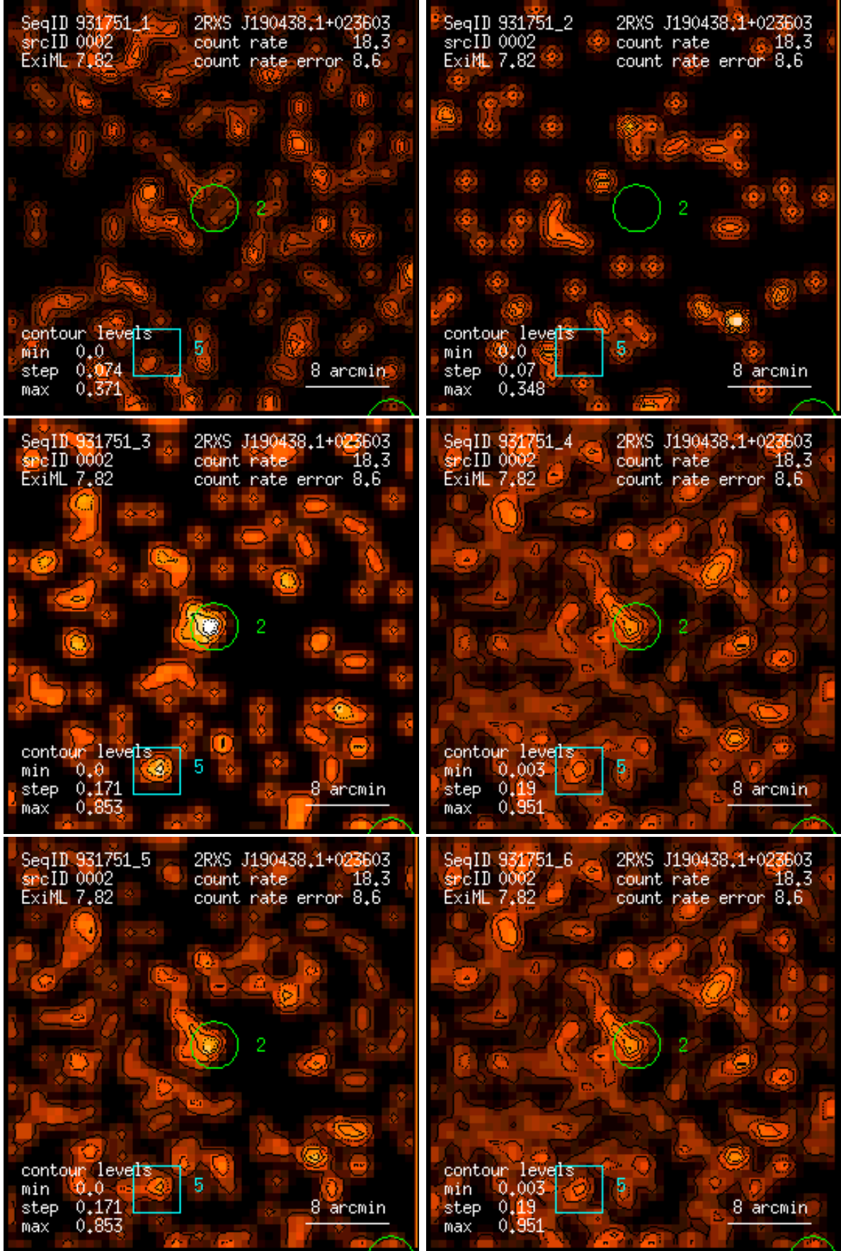
Figure 2: RASS 931751: detection 0002: band rate images, Gaussian filter: (1) PSPC channels 11 – 41, (2) 52 – 90, (3) 91 – 201, (4) 11 – 235, (5) 52 – 201, (6) 11 – 201. Broad band rates in counts/ks. Band rate contour levels in counts/ks/arcmin 2 .
