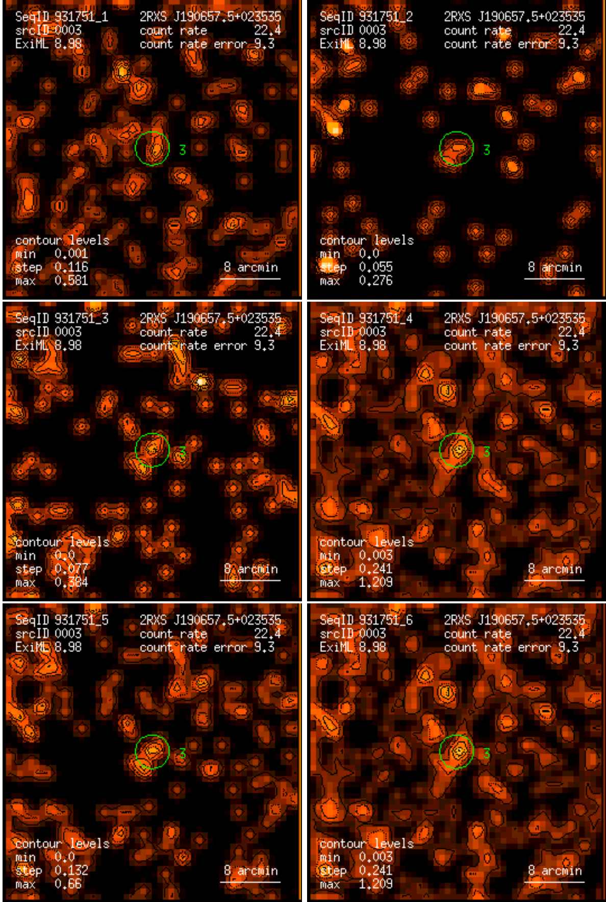
Figure 3: RASS 931751: detection 0003: band rate images, Gaussian filter: (1) PSPC channels 11 – 41, (2) 52 – 90, (3) 91 – 201, (4) 11 – 235, (5) 52 – 201, (6) 11 – 201. Broad band rates in counts/ks. Band rate contour levels in counts/ks/arcmin 2 .
