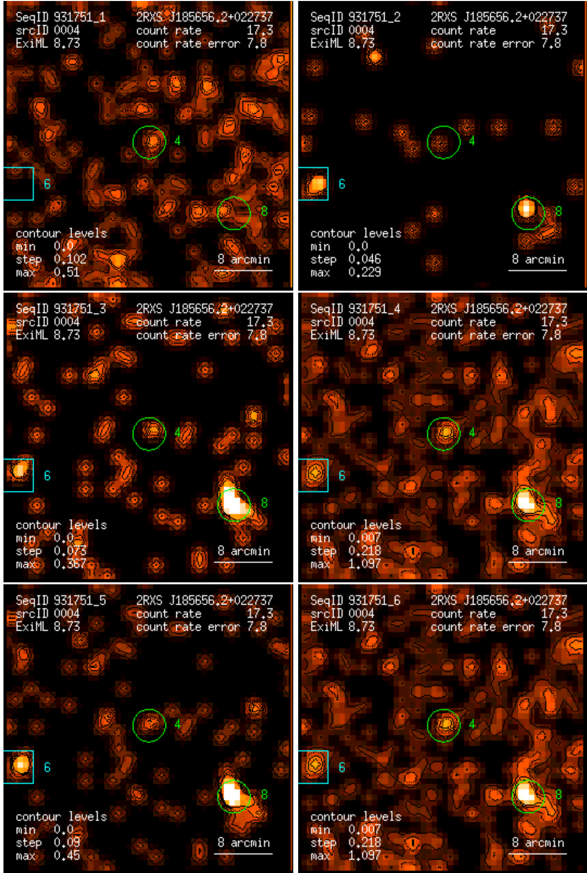
Figure 4: RASS 931751: detection 0004: band rate images, Gaussian filter: (1) PSPC channels 11 – 41, (2) 52 – 90, (3) 91 – 201, (4) 11 – 235, (5) 52 – 201, (6) 11 – 201. Broad band rates in counts/ks. Band rate contour levels in counts/ks/arcmin 2 .
