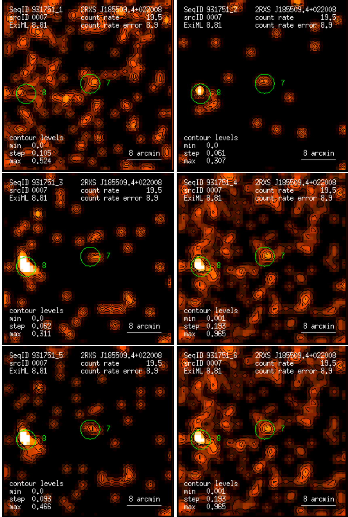
Figure 7: RASS 931751: detection 0007: band rate images, Gaussian filter: (1) PSPC channels 11 – 41, (2) 52 – 90, (3) 91 – 201, (4) 11 – 235, (5) 52 – 201, (6) 11 – 201. Broad band rates in counts/ks. Band rate contour levels in counts/ks/arcmin 2 .
