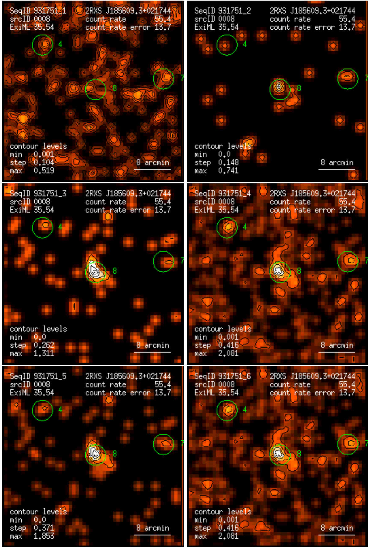
Figure 8: RASS 931751: detection 0008: band rate images, Gaussian filter: (1) PSPC channels 11 – 41, (2) 52 – 90, (3) 91 – 201, (4) 11 – 235, (5) 52 – 201, (6) 11 – 201. Broad band rates in counts/ks. Band rate contour levels in counts/ks/arcmin 2 .
