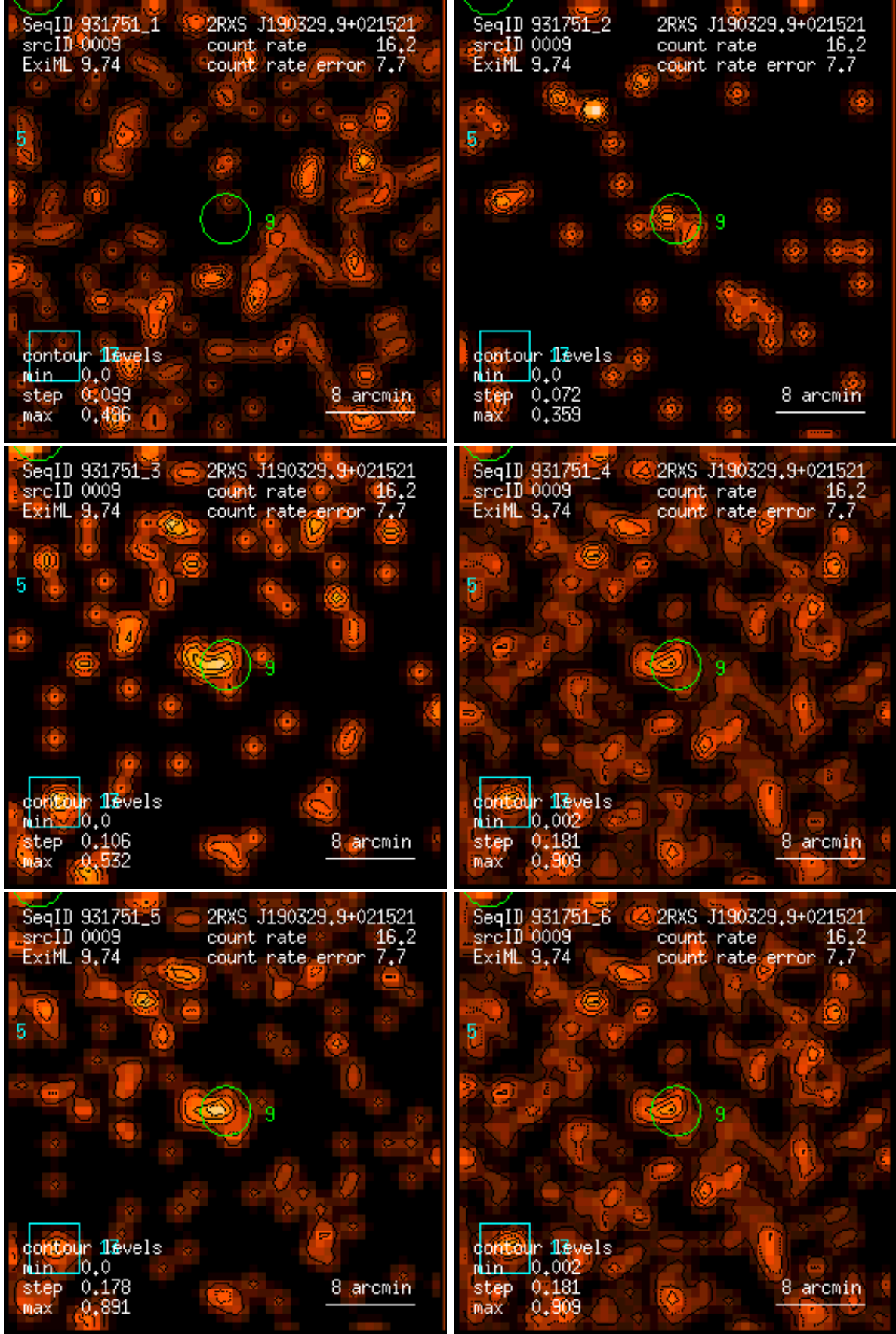
Figure 9: RASS 931751: detection 0009: band rate images, Gaussian filter: (1) PSPC channels 11 – 41, (2) 52 – 90, (3) 91 – 201, (4) 11 – 235, (5) 52 – 201, (6) 11 – 201. Broad band rates in counts/ks. Band rate contour levels in counts/ks/arcmin 2 .
