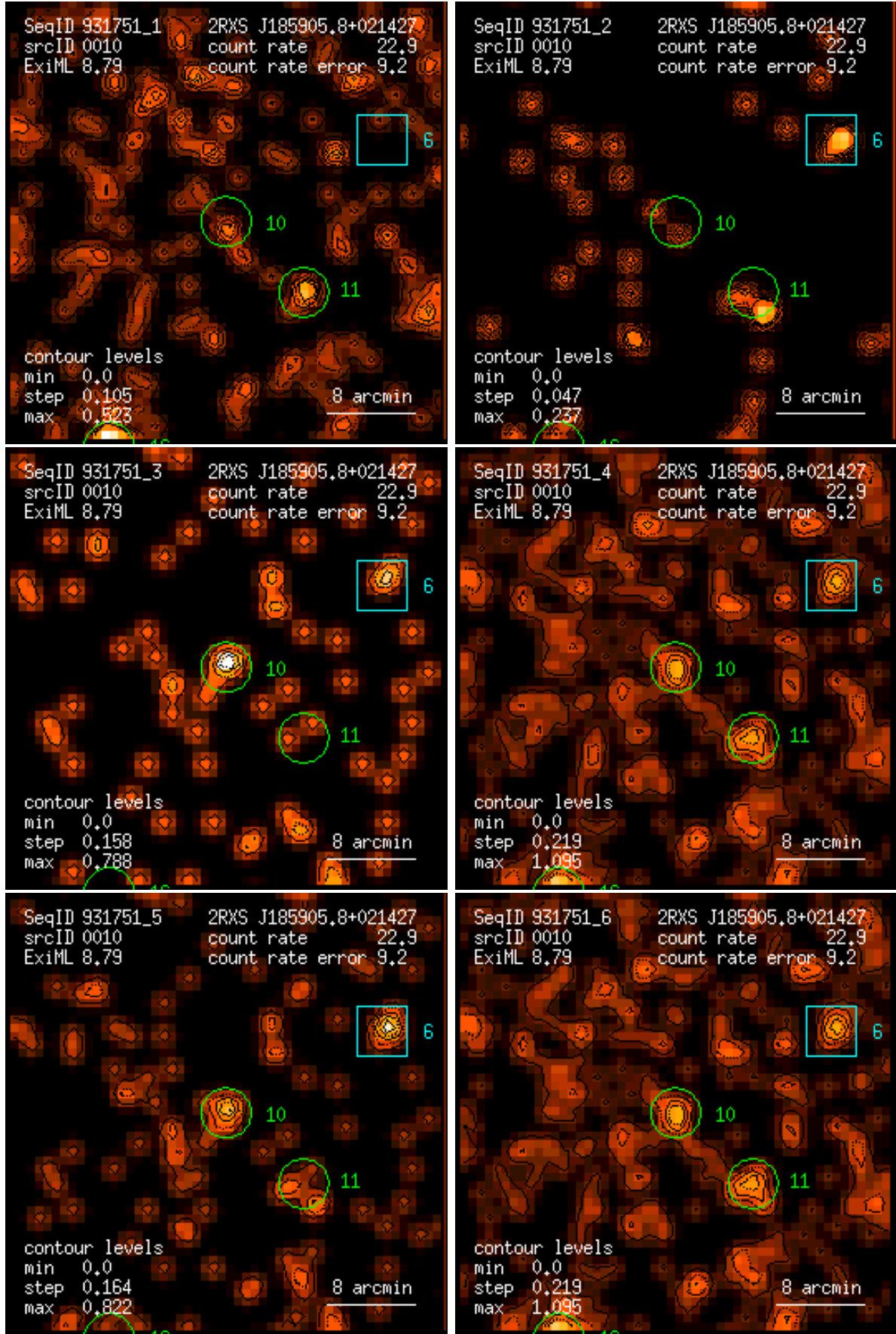
Figure 10: RASS 931751: detection 0010: band rate images, Gaussian filter: (1) PSPC channels 11 – 41, (2) 52 – 90, (3) 91 – 201, (4) 11 – 235, (5) 52 – 201, (6) 11 – 201. Broad band rates in counts/ks. Band rate contour levels in counts/ks/arcmin 2 .
