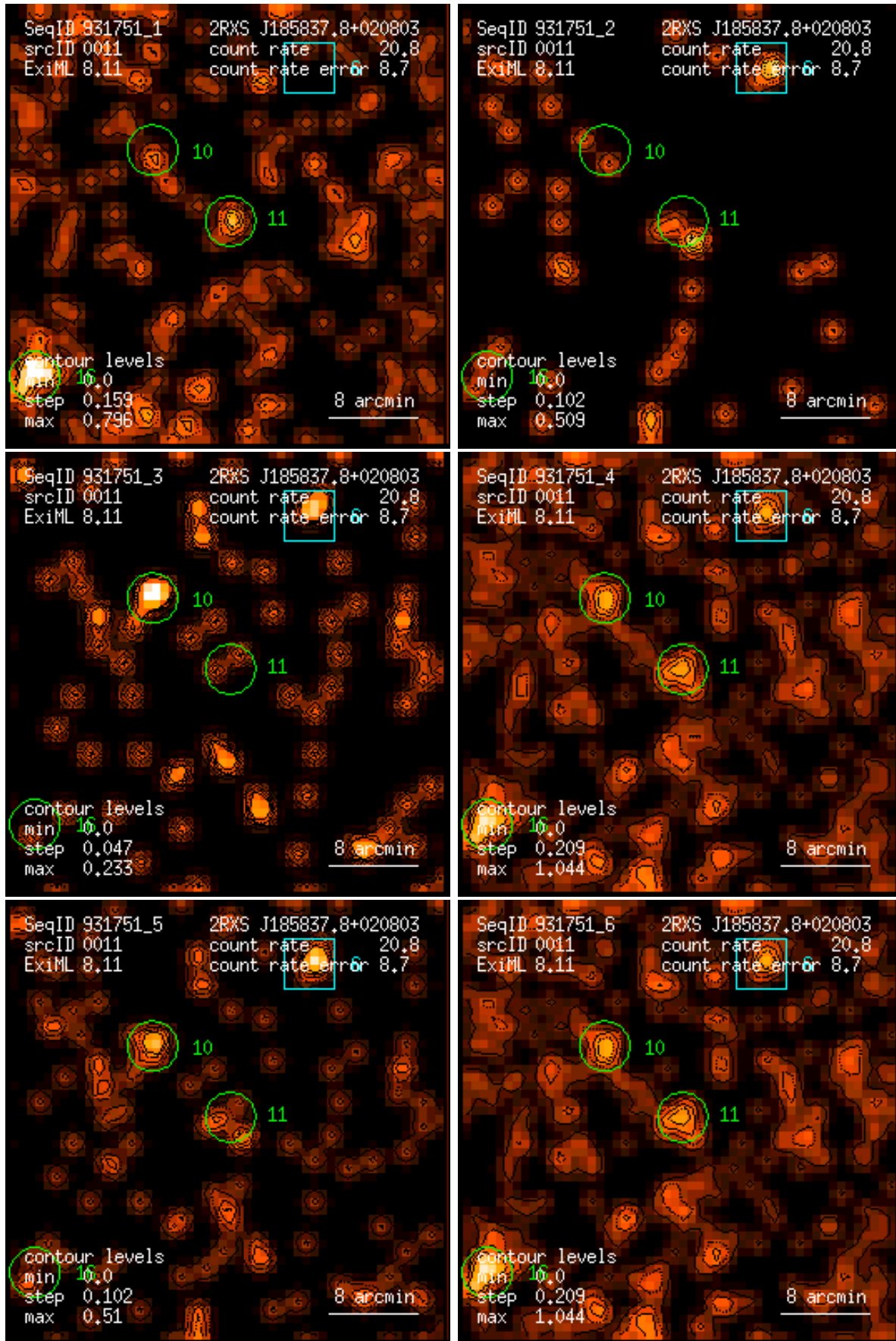
Figure 11: RASS 931751: detection 0011: band rate images, Gaussian filter: (1) PSPC channels 11 – 41, (2) 52 – 90, (3) 91 – 201, (4) 11 – 235, (5) 52 – 201, (6) 11 – 201. Broad band rates in counts/ks. Band rate contour levels in counts/ks/arcmin 2 .
