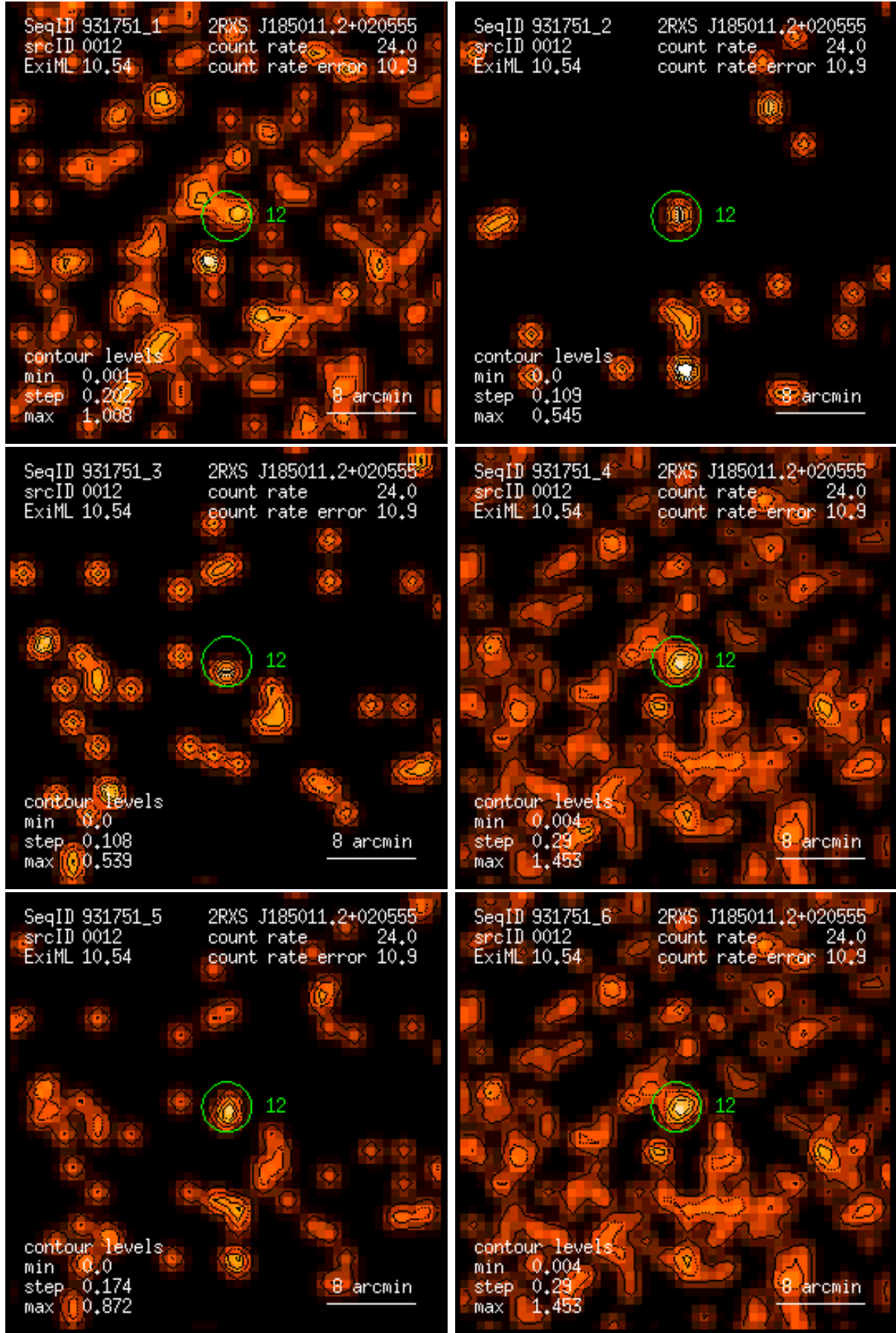
Figure 12: RASS 931751: detection 0012: band rate images, Gaussian filter: (1) PSPC channels 11 – 41, (2) 52 – 90, (3) 91 – 201, (4) 11 – 235, (5) 52 – 201, (6) 11 – 201. Broad band rates in counts/ks. Band rate contour levels in counts/ks/arcmin 2 .
