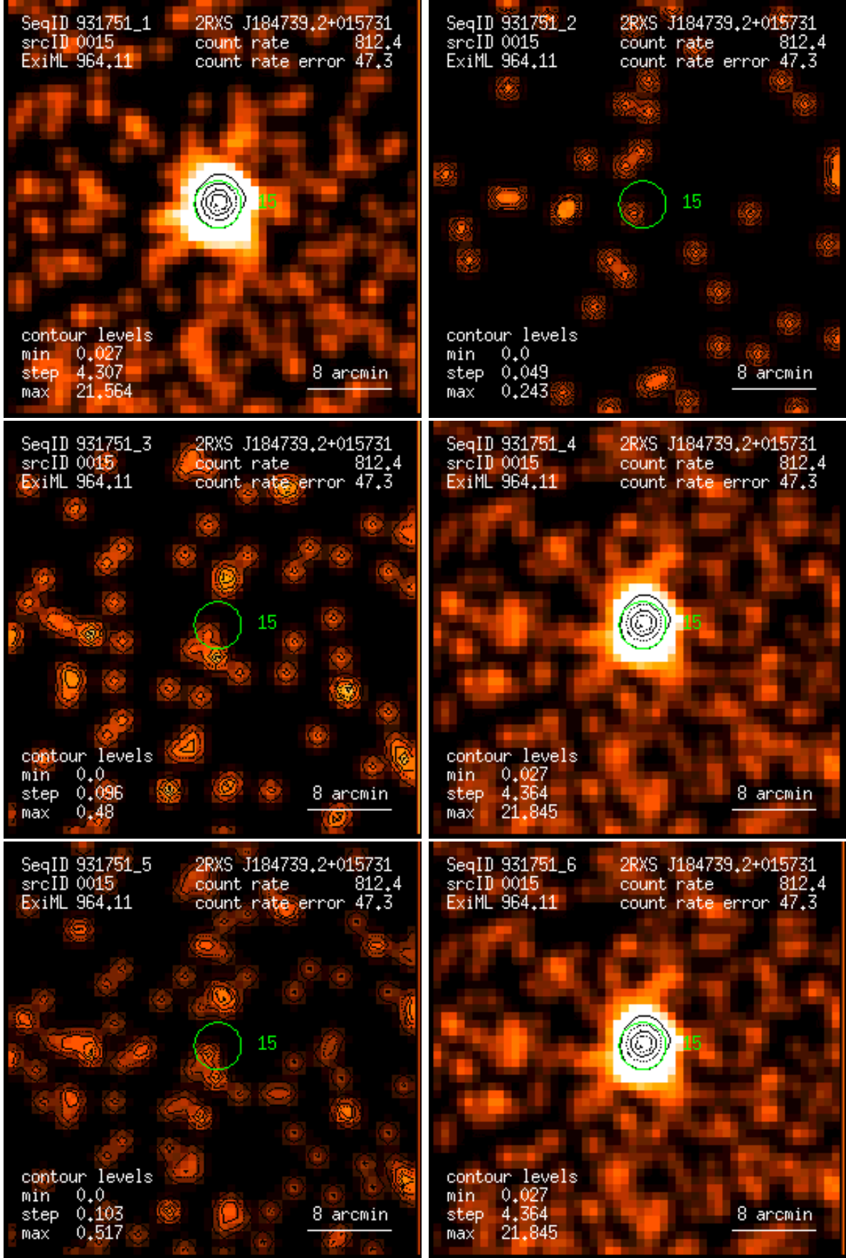
Figure 15: RASS 931751: detection 0015: band rate images, Gaussian filter: (1) PSPC channels 11 – 41, (2) 52 – 90, (3) 91 – 201, (4) 11 – 235, (5) 52 – 201, (6) 11 – 201. Broad band rates in counts/ks. Band rate contour levels in counts/ks/arcmin 2 .
