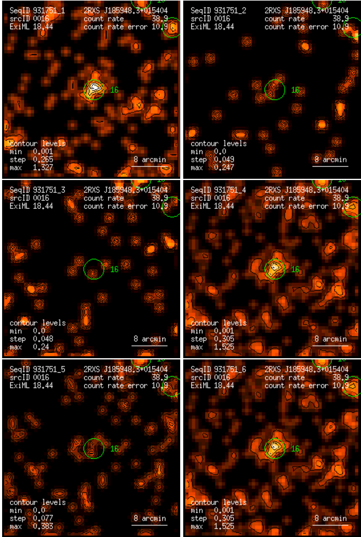
Figure 16: RASS 931751: detection 0016: band rate images, Gaussian filter: (1) PSPC channels 11 – 41, (2) 52 – 90, (3) 91 – 201, (4) 11 – 235, (5) 52 – 201, (6) 11 – 201. Broad band rates in counts/ks. Band rate contour levels in counts/ks/arcmin 2 .
