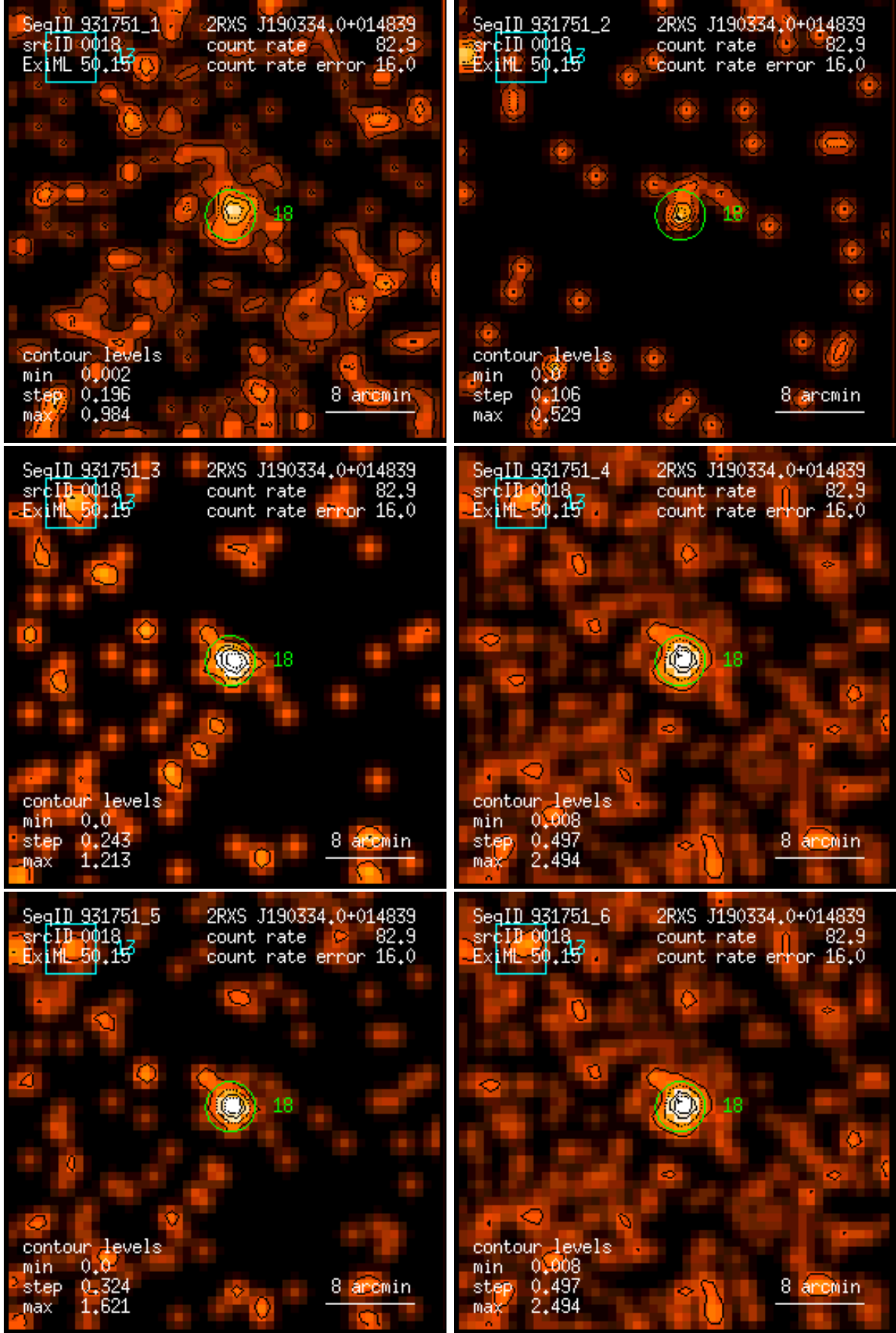
Figure 18: RASS 931751: detection 0018: band rate images, Gaussian filter: (1) PSPC channels 11 – 41, (2) 52 – 90, (3) 91 – 201, (4) 11 – 235, (5) 52 – 201, (6) 11 – 201. Broad band rates in counts/ks. Band rate contour levels in counts/ks/arcmin 2 .
