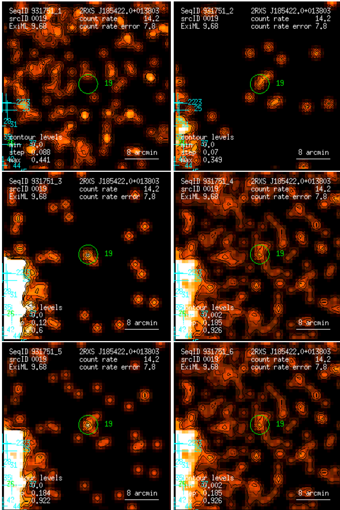
Figure 19: RASS 931751: detection 0019: band rate images, Gaussian filter: (1) PSPC channels 11 – 41, (2) 52 – 90, (3) 91 – 201, (4) 11 – 235, (5) 52 – 201, (6) 11 – 201. Broad band rates in counts/ks. Band rate contour levels in counts/ks/arcmin 2 .
