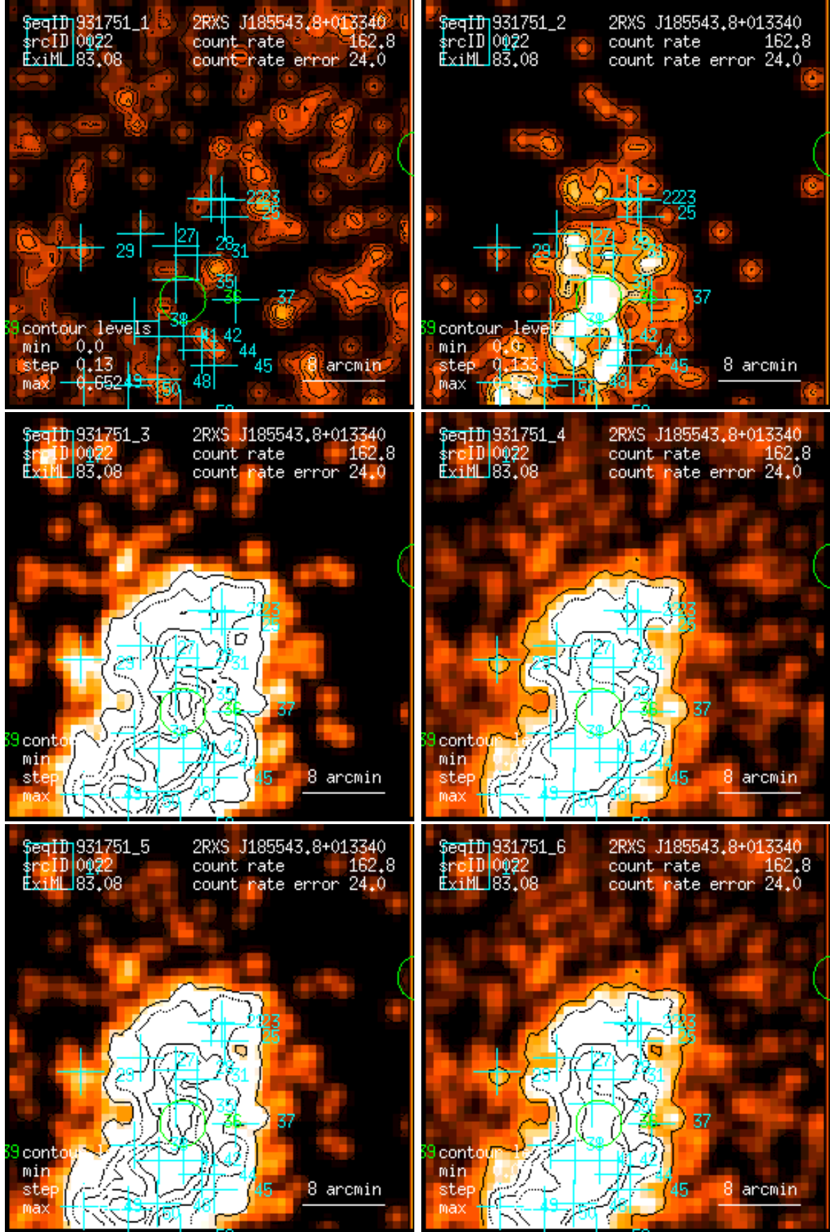
Figure 22: RASS 931751: detection 0022: band rate images, Gaussian filter: (1) PSPC channels 11 – 41, (2) 52 – 90, (3) 91 – 201, (4) 11 – 235, (5) 52 – 201, (6) 11 – 201. Broad band rates in counts/ks. Band rate contour levels in counts/ks/arcmin 2 .
