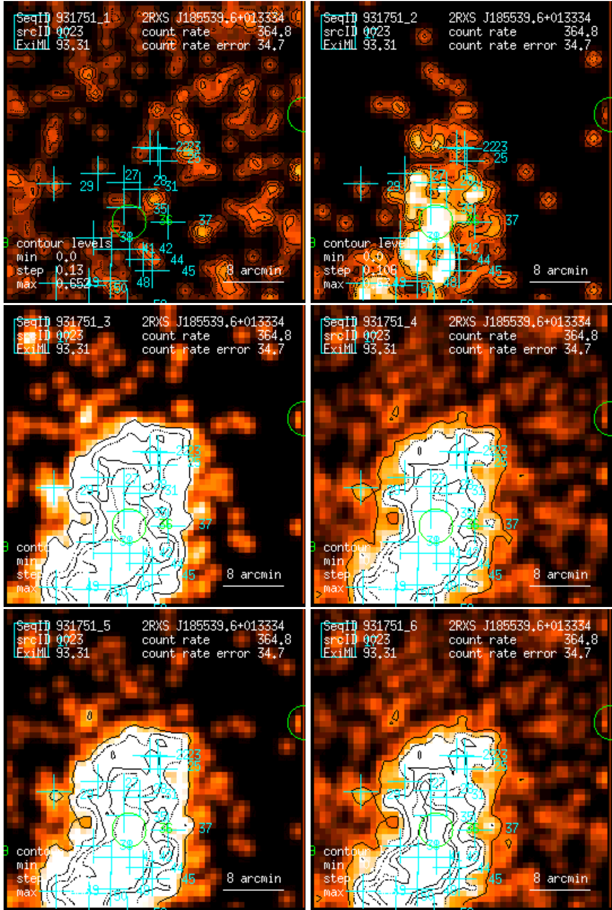
Figure 23: RASS 931751: detection 0023: band rate images, Gaussian filter: (1) PSPC channels 11 – 41, (2) 52 – 90, (3) 91 – 201, (4) 11 – 235, (5) 52 – 201, (6) 11 – 201. Broad band rates in counts/ks. Band rate contour levels in counts/ks/arcmin 2 .
