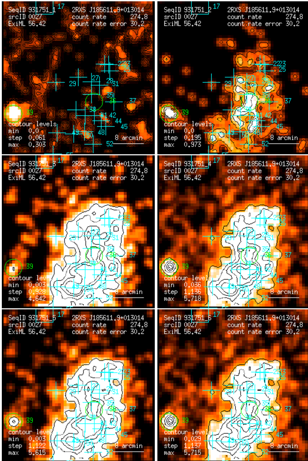
Figure 27: RASS 931751: detection 0027: band rate images, Gaussian filter: (1) PSPC channels 11 – 41, (2) 52 – 90, (3) 91 – 201, (4) 11 – 235, (5) 52 – 201, (6) 11 – 201. Broad band rates in counts/ks. Band rate contour levels in counts/ks/arcmin 2 .
