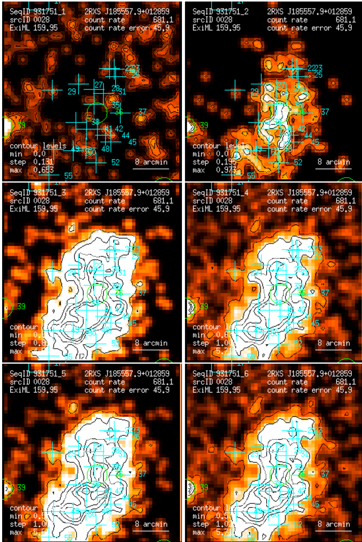
Figure 28: RASS 931751: detection 0028: band rate images, Gaussian filter: (1) PSPC channels 11 – 41, (2) 52 – 90, (3) 91 – 201, (4) 11 – 235, (5) 52 – 201, (6) 11 – 201. Broad band rates in counts/ks. Band rate contour levels in counts/ks/arcmin 2 .
