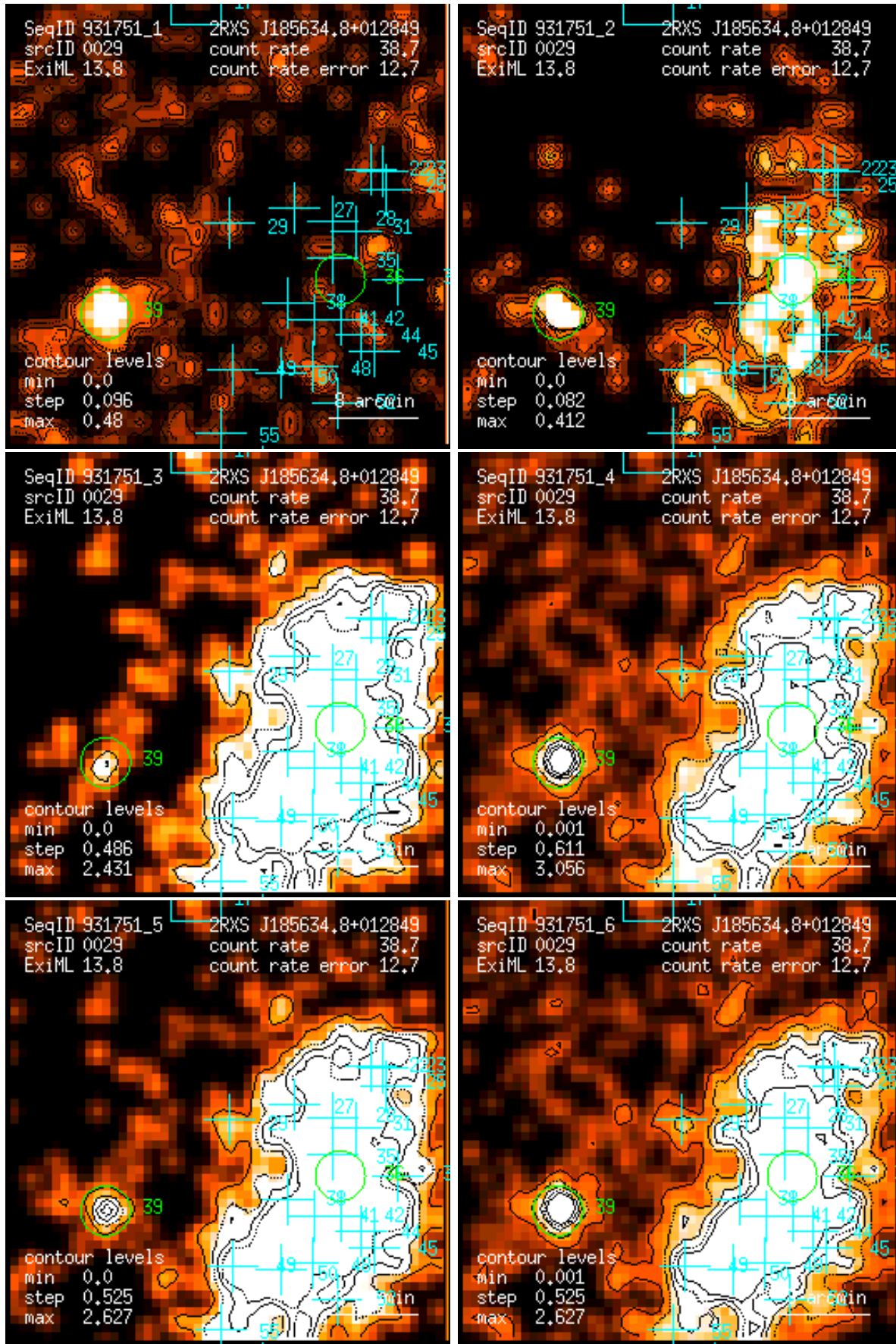
Figure 29: RASS 931751: detection 0029: band rate images, Gaussian filter: (1) PSPC channels 11 – 41, (2) 52 – 90, (3) 91 – 201, (4) 11 – 235, (5) 52 – 201, (6) 11 – 201. Broad band rates in counts/ks. Band rate contour levels in counts/ks/arcmin 2 .
