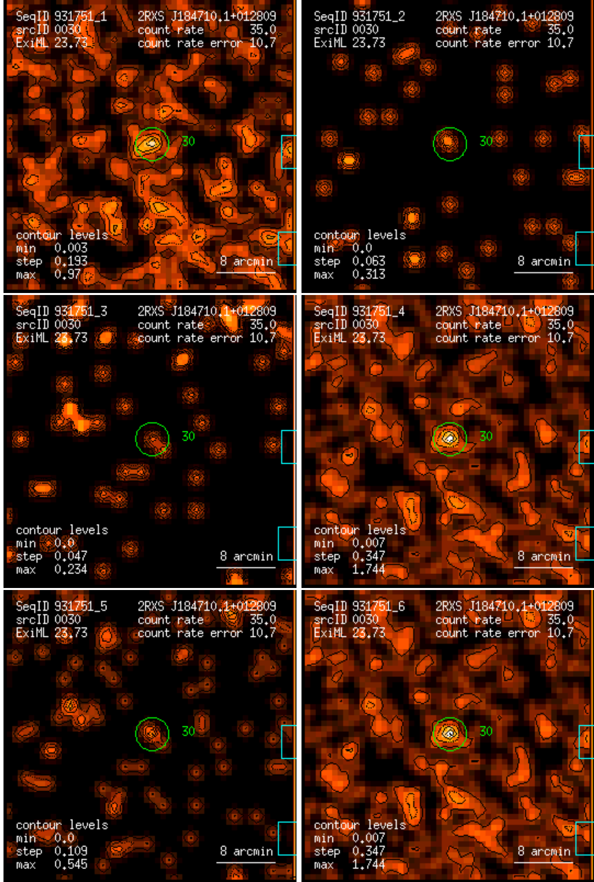
Figure 30: RASS 931751: detection 0030: band rate images, Gaussian filter: (1) PSPC channels 11 – 41, (2) 52 – 90, (3) 91 – 201, (4) 11 – 235, (5) 52 – 201, (6) 11 – 201. Broad band rates in counts/ks. Band rate contour levels in counts/ks/arcmin 2 .
