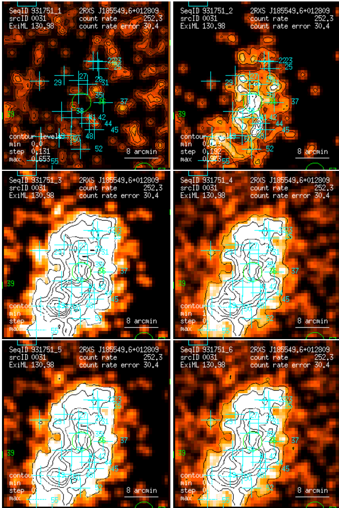
Figure 31: RASS 931751: detection 0031: band rate images, Gaussian filter: (1) PSPC channels 11 – 41, (2) 52 – 90, (3) 91 – 201, (4) 11 – 235, (5) 52 – 201, (6) 11 – 201. Broad band rates in counts/ks. Band rate contour levels in counts/ks/arcmin 2 .
