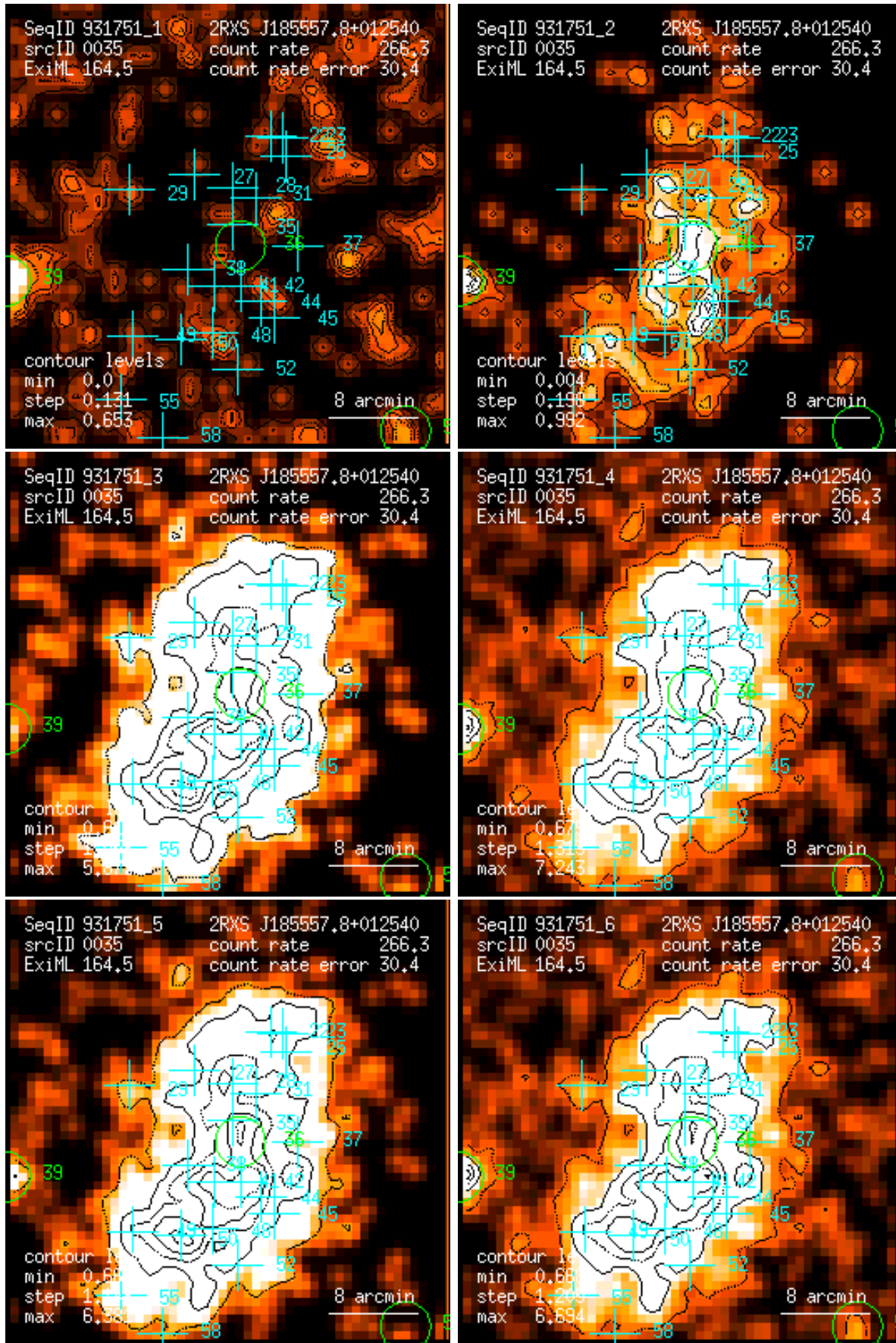
Figure 35: RASS 931751: detection 0035: band rate images, Gaussian filter: (1) PSPC channels 11 – 41, (2) 52 – 90, (3) 91 – 201, (4) 11 – 235, (5) 52 – 201, (6) 11 – 201. Broad band rates in counts/ks. Band rate contour levels in counts/ks/arcmin 2 .
