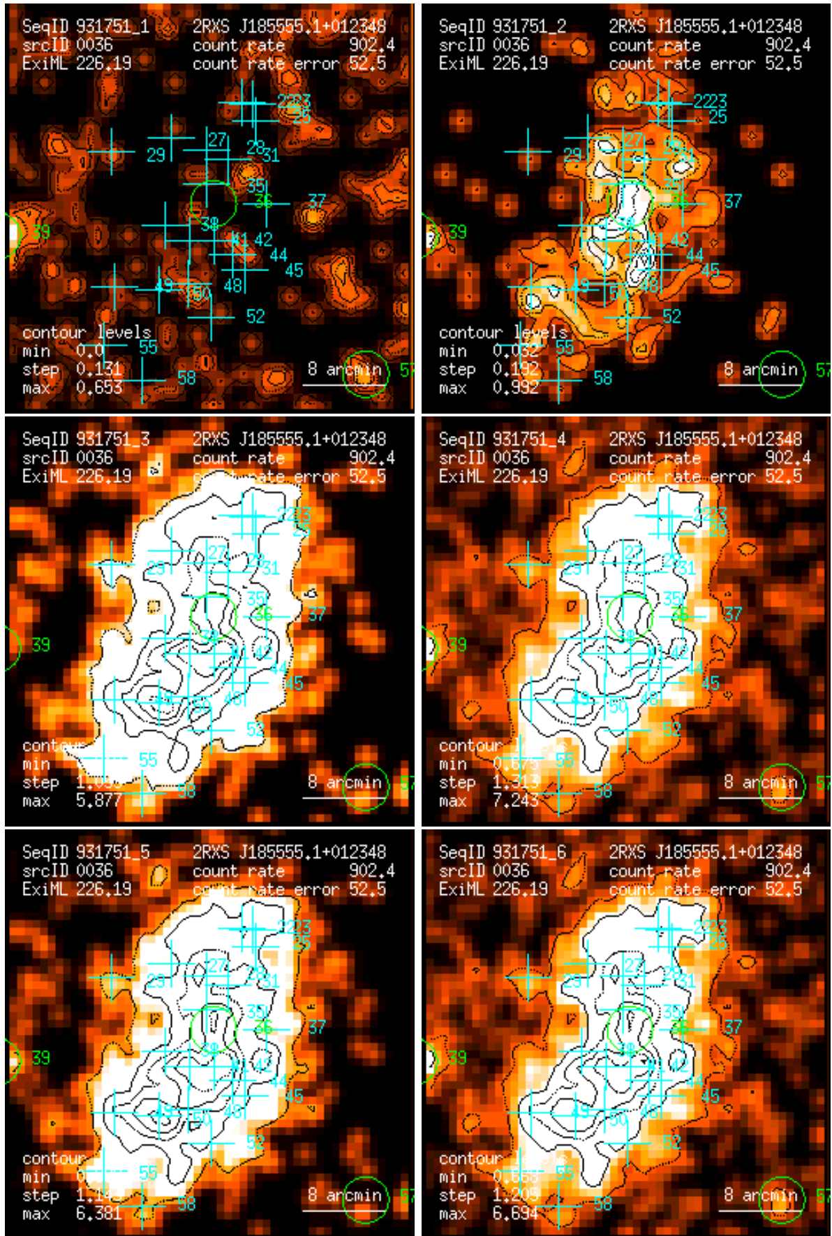
Figure 36: RASS 931751: detection 0036: band rate images, Gaussian filter: (1) PSPC channels 11 – 41, (2) 52 – 90, (3) 91 – 201, (4) 11 – 235, (5) 52 – 201, (6) 11 – 201. Broad band rates in counts/ks. Band rate contour levels in counts/ks/arcmin 2 .
