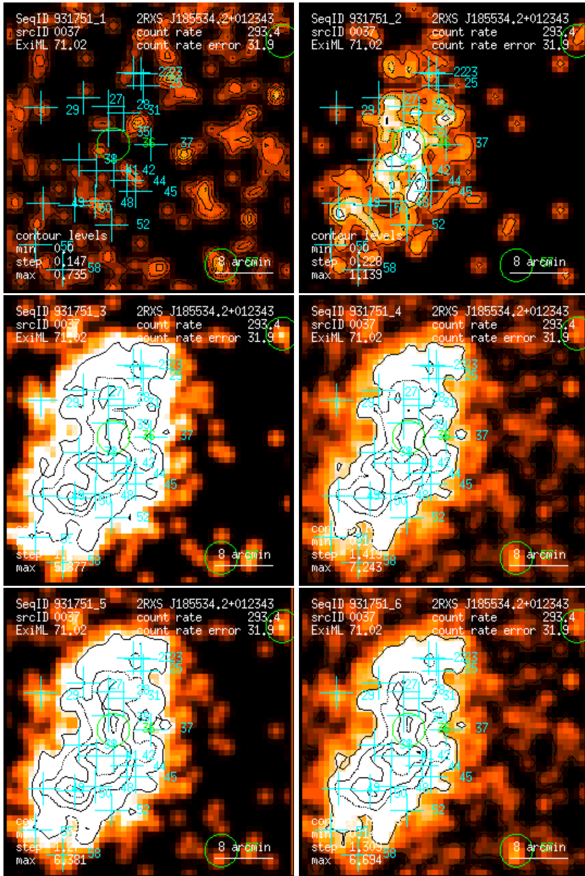
Figure 37: RASS 931751: detection 0037: band rate images, Gaussian filter: (1) PSPC channels 11 – 41, (2) 52 – 90, (3) 91 – 201, (4) 11 – 235, (5) 52 – 201, (6) 11 – 201. Broad band rates in counts/ks. Band rate contour levels in counts/ks/arcmin 2 .
