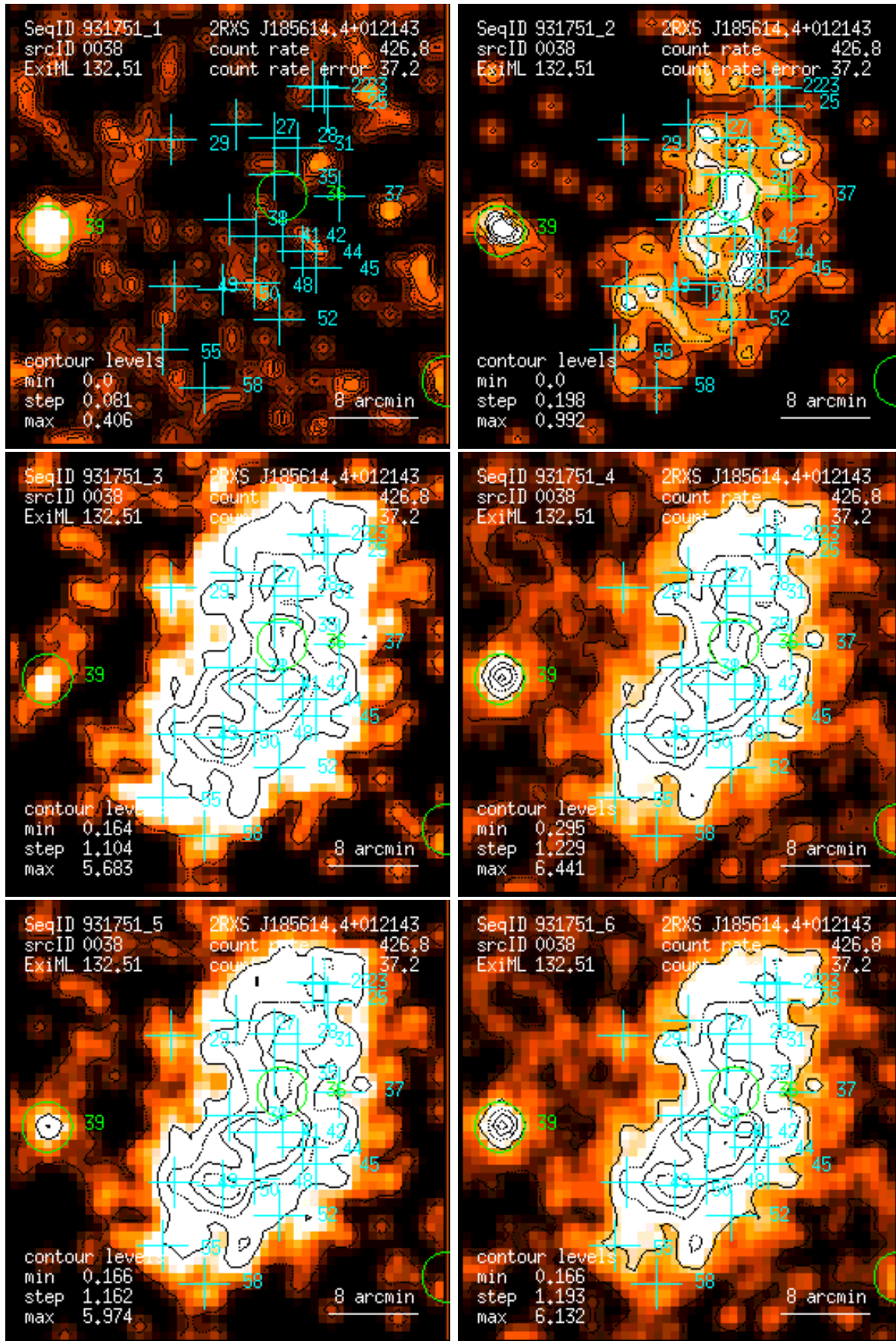
Figure 38: RASS 931751: detection 0038: band rate images, Gaussian filter: (1) PSPC channels 11 – 41, (2) 52 – 90, (3) 91 – 201, (4) 11 – 235, (5) 52 – 201, (6) 11 – 201. Broad band rates in counts/ks. Band rate contour levels in counts/ks/arcmin 2 .
