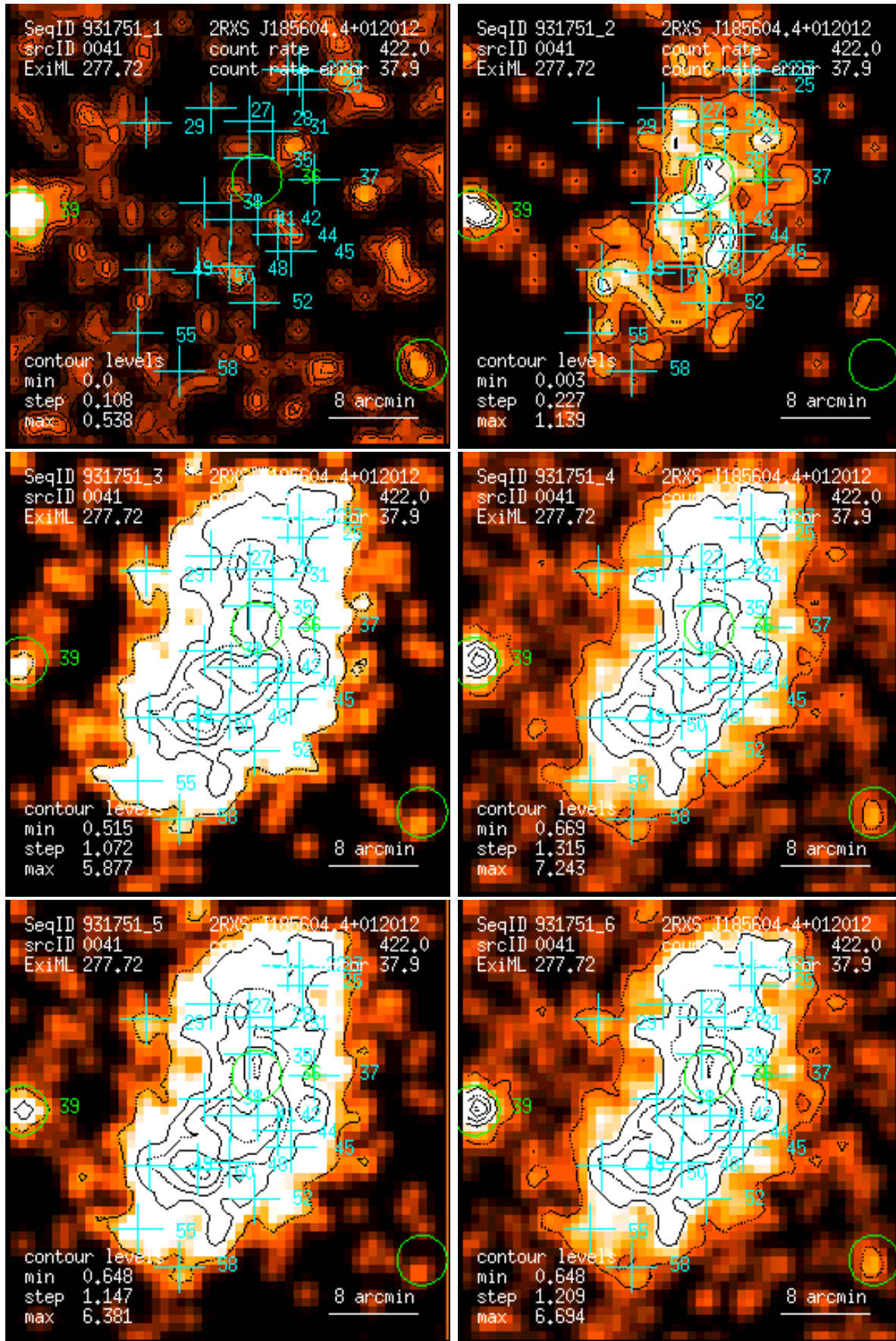
Figure 41: RASS 931751: detection 0041: band rate images, Gaussian filter: (1) PSPC channels 11 – 41, (2) 52 – 90, (3) 91 – 201, (4) 11 – 235, (5) 52 – 201, (6) 11 – 201. Broad band rates in counts/ks. Band rate contour levels in counts/ks/arcmin 2 .
