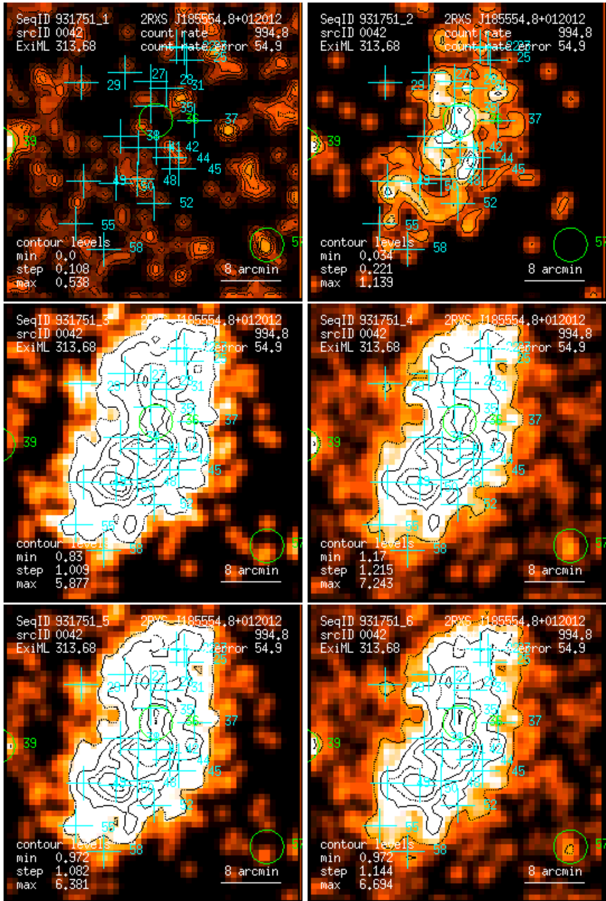
Figure 42: RASS 931751: detection 0042: band rate images, Gaussian filter: (1) PSPC channels 11 – 41, (2) 52 – 90, (3) 91 – 201, (4) 11 – 235, (5) 52 – 201, (6) 11 – 201. Broad band rates in counts/ks. Band rate contour levels in counts/ks/arcmin 2 .
