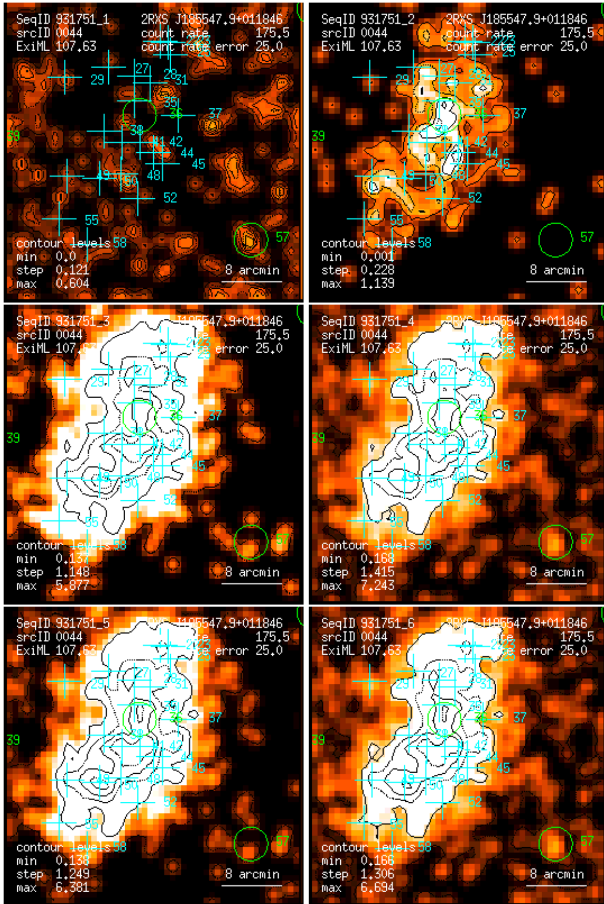
Figure 44: RASS 931751: detection 0044: band rate images, Gaussian filter: (1) PSPC channels 11 – 41, (2) 52 – 90, (3) 91 – 201, (4) 11 – 235, (5) 52 – 201, (6) 11 – 201. Broad band rates in counts/ks. Band rate contour levels in counts/ks/arcmin 2 .
