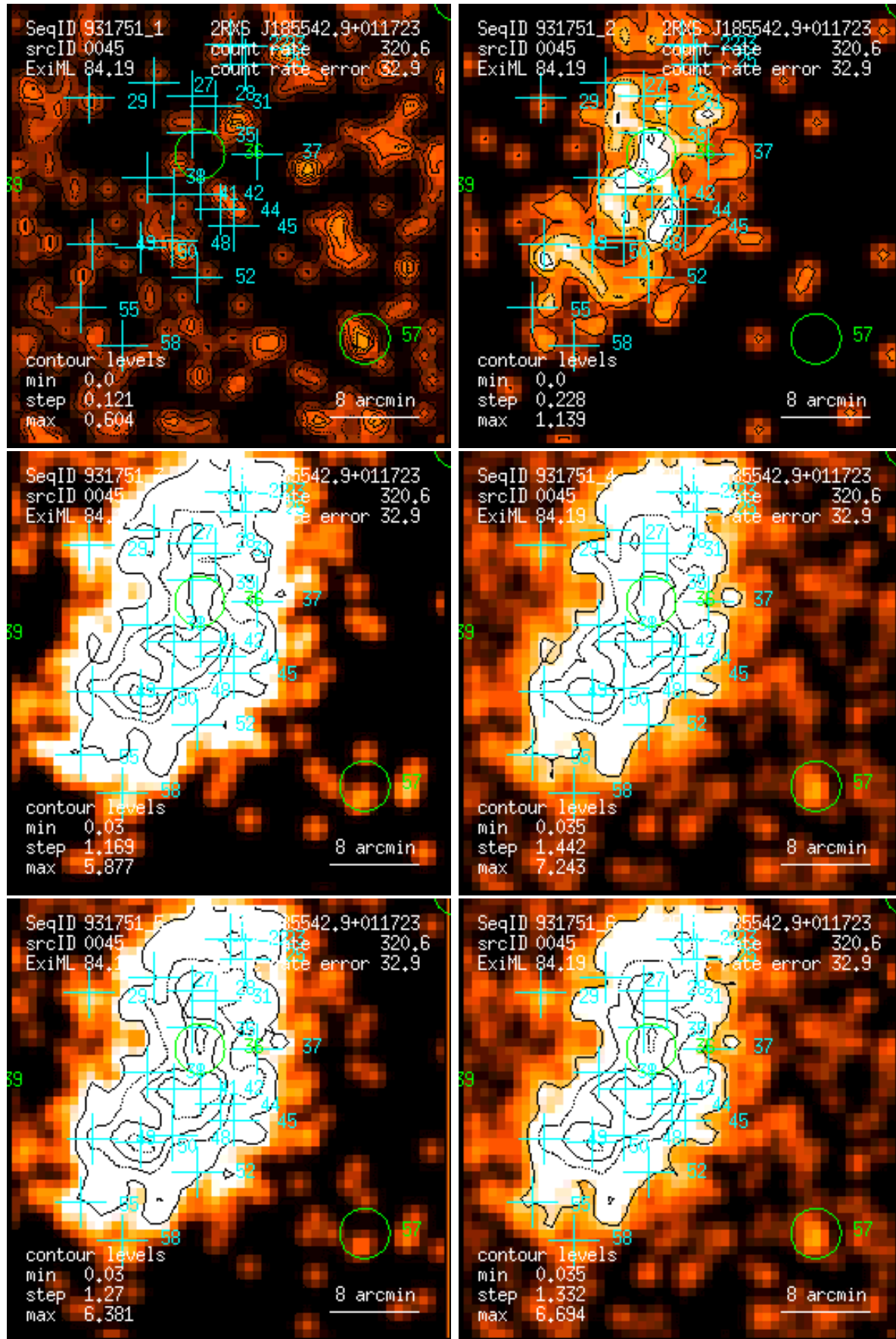
Figure 45: RASS 931751: detection 0045: band rate images, Gaussian filter: (1) PSPC channels 11 – 41, (2) 52 – 90, (3) 91 – 201, (4) 11 – 235, (5) 52 – 201, (6) 11 – 201. Broad band rates in counts/ks. Band rate contour levels in counts/ks/arcmin 2 .
