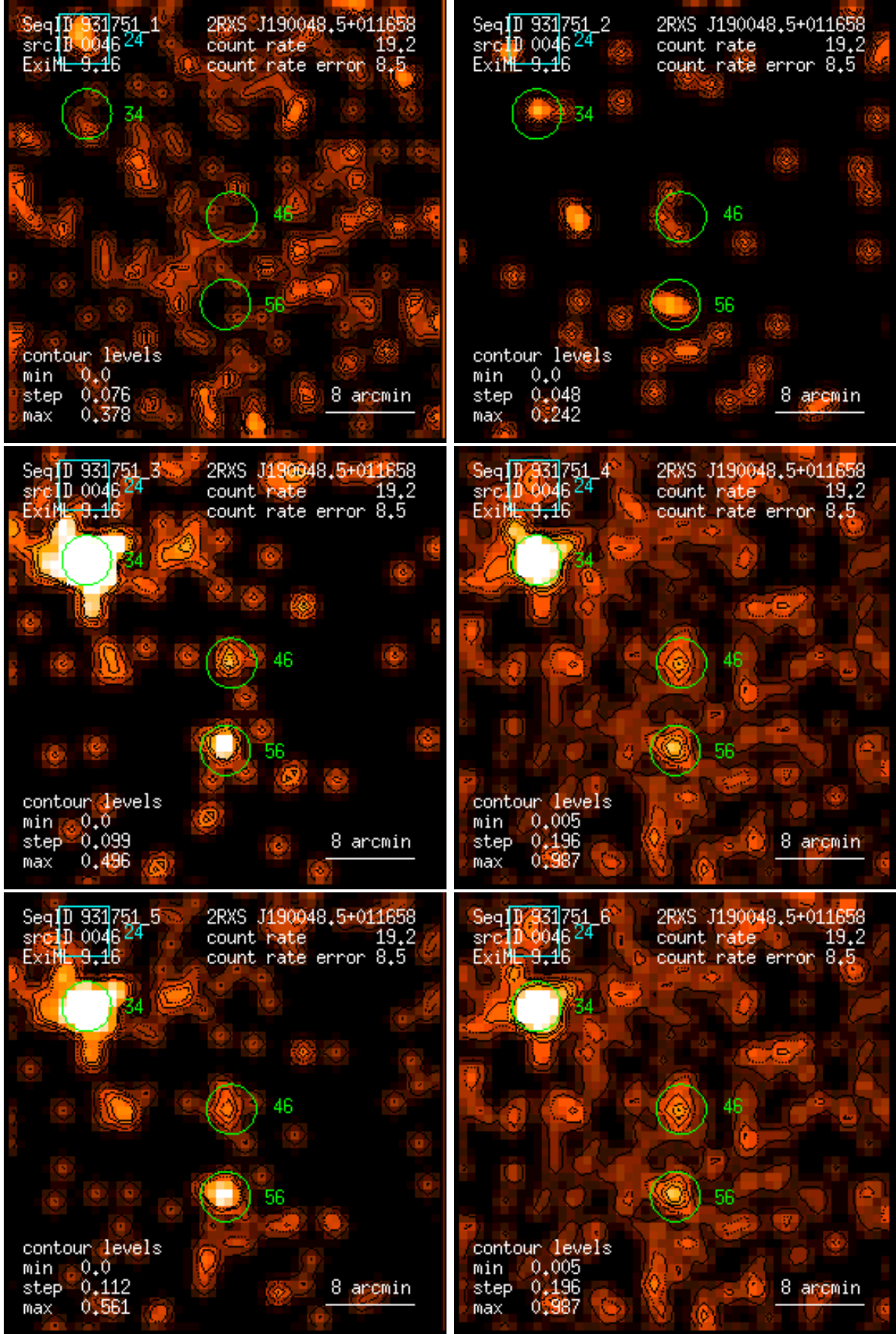
Figure 46: RASS 931751: detection 0046: band rate images, Gaussian filter: (1) PSPC channels 11 – 41, (2) 52 – 90, (3) 91 – 201, (4) 11 – 235, (5) 52 – 201, (6) 11 – 201. Broad band rates in counts/ks. Band rate contour levels in counts/ks/arcmin 2 .
