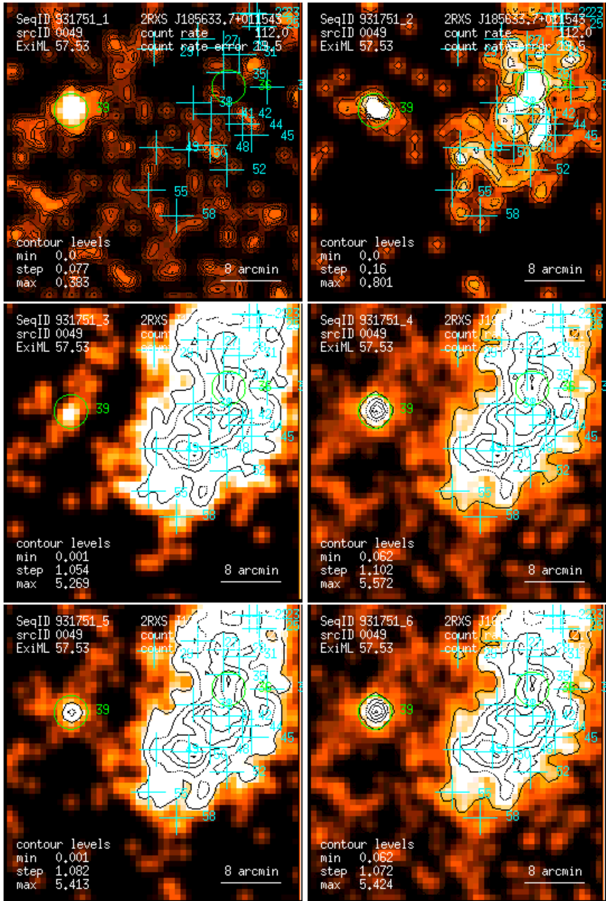
Figure 49: RASS 931751: detection 0049: band rate images, Gaussian filter: (1) PSPC channels 11 – 41, (2) 52 – 90, (3) 91 – 201, (4) 11 – 235, (5) 52 – 201, (6) 11 – 201. Broad band rates in counts/ks. Band rate contour levels in counts/ks/arcmin 2 .
