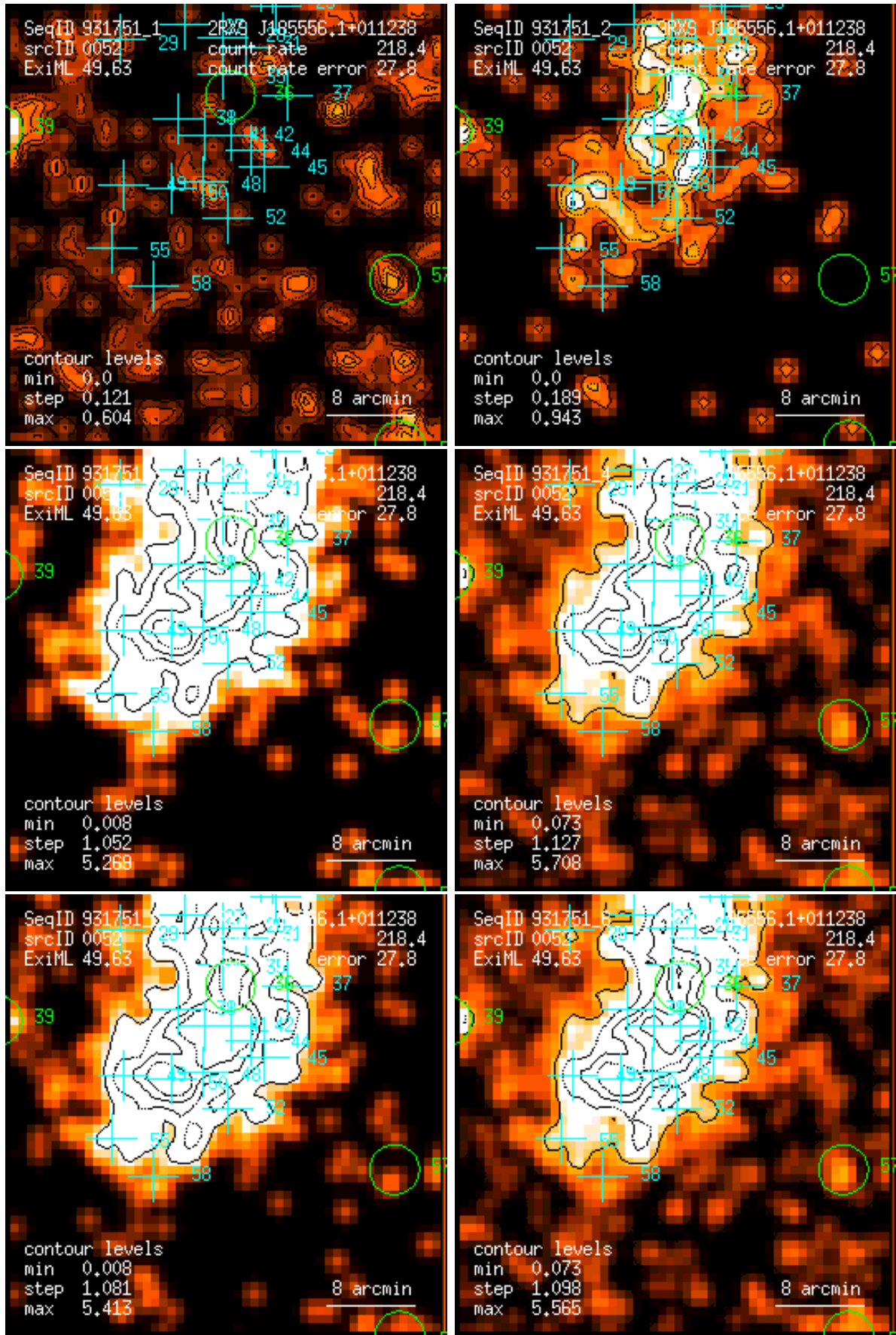
Figure 52: RASS 931751: detection 0052: band rate images, Gaussian filter: (1) PSPC channels 11 – 41, (2) 52 – 90, (3) 91 – 201, (4) 11 – 235, (5) 52 – 201, (6) 11 – 201. Broad band rates in counts/ks. Band rate contour levels in counts/ks/arcmin 2 .
