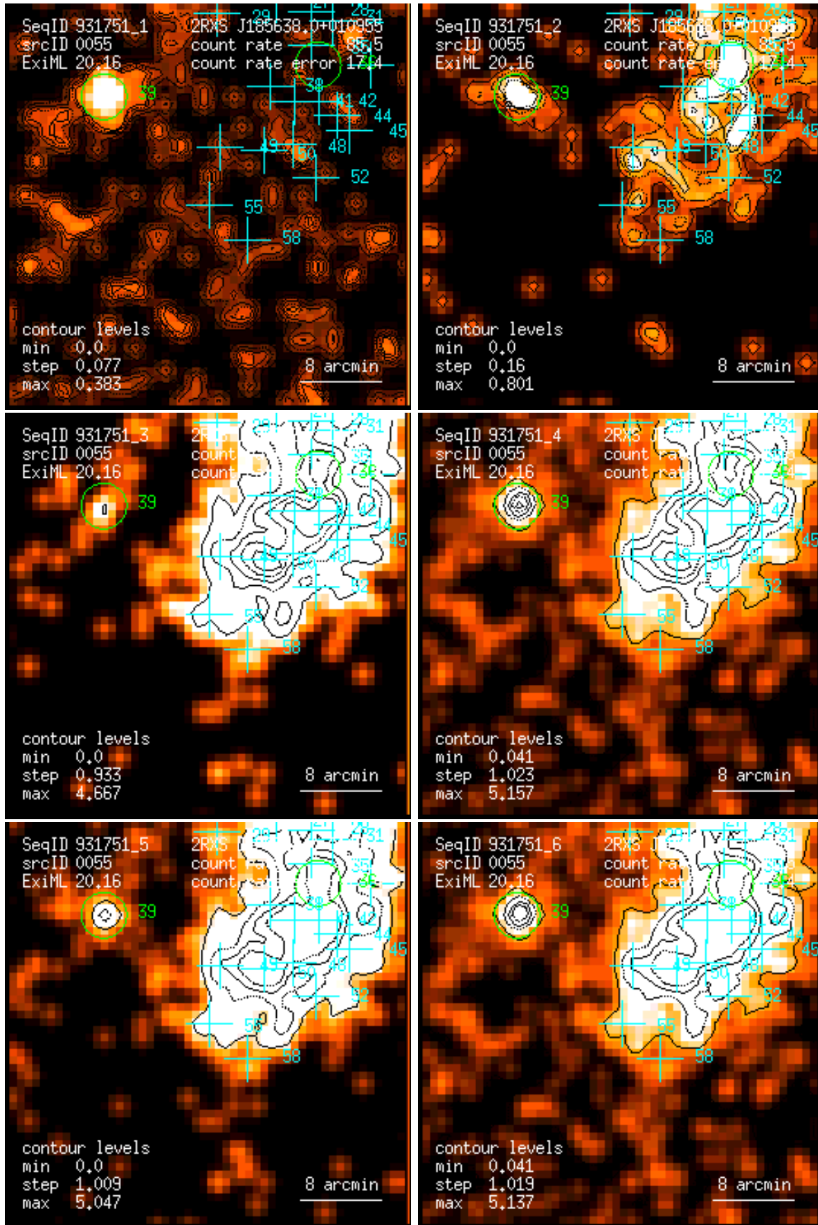
Figure 55: RASS 931751: detection 0055: band rate images, Gaussian filter: (1) PSPC channels 11 – 41, (2) 52 – 90, (3) 91 – 201, (4) 11 – 235, (5) 52 – 201, (6) 11 – 201. Broad band rates in counts/ks. Band rate contour levels in counts/ks/arcmin 2 .
