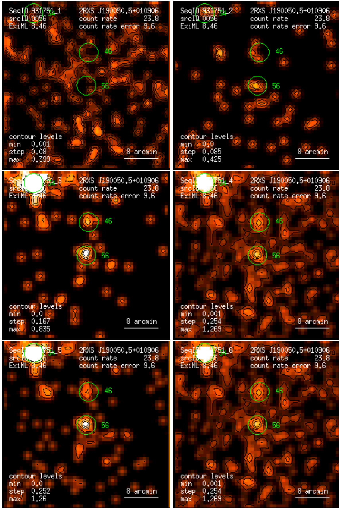
Figure 56: RASS 931751: detection 0056: band rate images, Gaussian filter: (1) PSPC channels 11 – 41, (2) 52 – 90, (3) 91 – 201, (4) 11 – 235, (5) 52 – 201, (6) 11 – 201. Broad band rates in counts/ks. Band rate contour levels in counts/ks/arcmin 2 .
