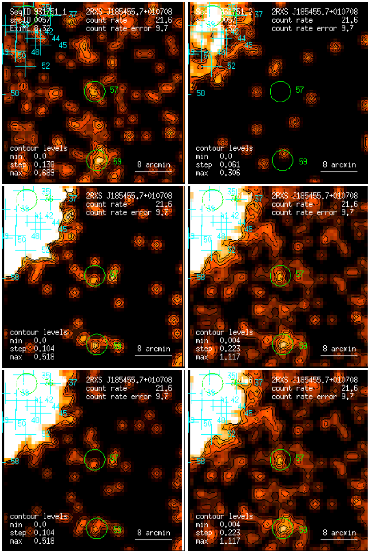
Figure 57: RASS 931751: detection 0057: band rate images, Gaussian filter: (1) PSPC channels 11 – 41, (2) 52 – 90, (3) 91 – 201, (4) 11 – 235, (5) 52 – 201, (6) 11 – 201. Broad band rates in counts/ks. Band rate contour levels in counts/ks/arcmin 2 .
