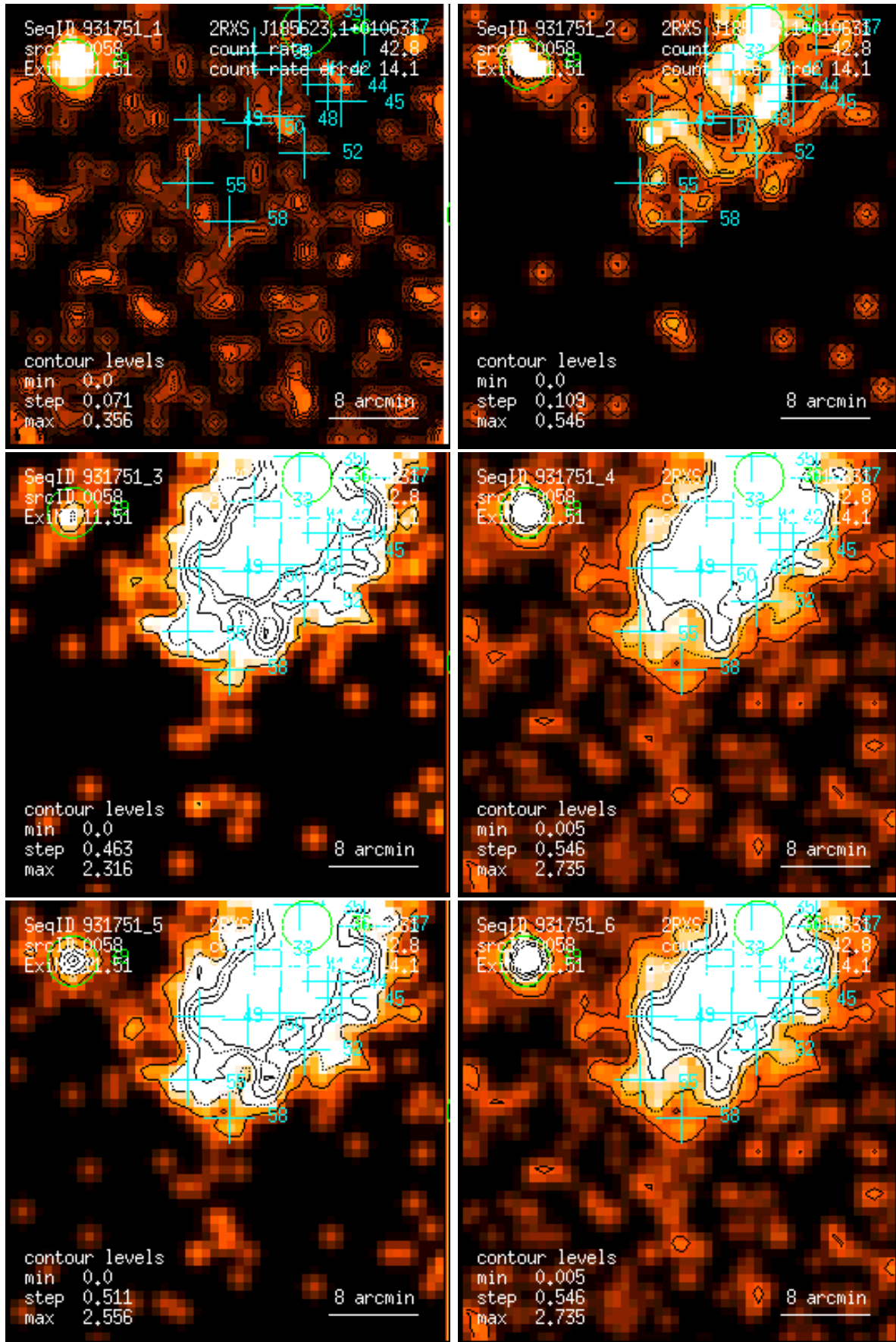
Figure 58: RASS 931751: detection 0058: band rate images, Gaussian filter: (1) PSPC channels 11 – 41, (2) 52 – 90, (3) 91 – 201, (4) 11 – 235, (5) 52 – 201, (6) 11 – 201. Broad band rates in counts/ks. Band rate contour levels in counts/ks/arcmin 2 .
