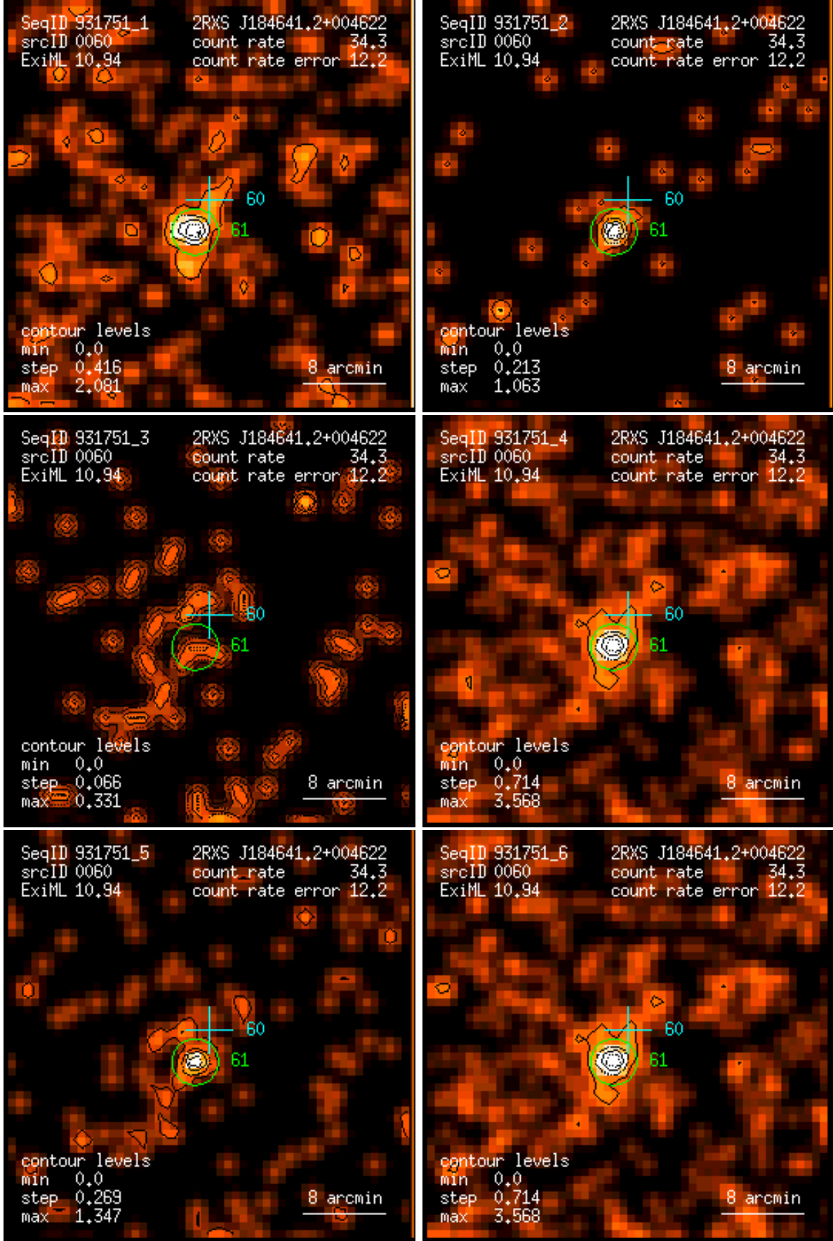
Figure 60: RASS 931751: detection 0060: band rate images, Gaussian filter: (1) PSPC channels 11 – 41, (2) 52 – 90, (3) 91 – 201, (4) 11 – 235, (5) 52 – 201, (6) 11 – 201. Broad band rates in counts/ks. Band rate contour levels in counts/ks/arcmin 2 .
