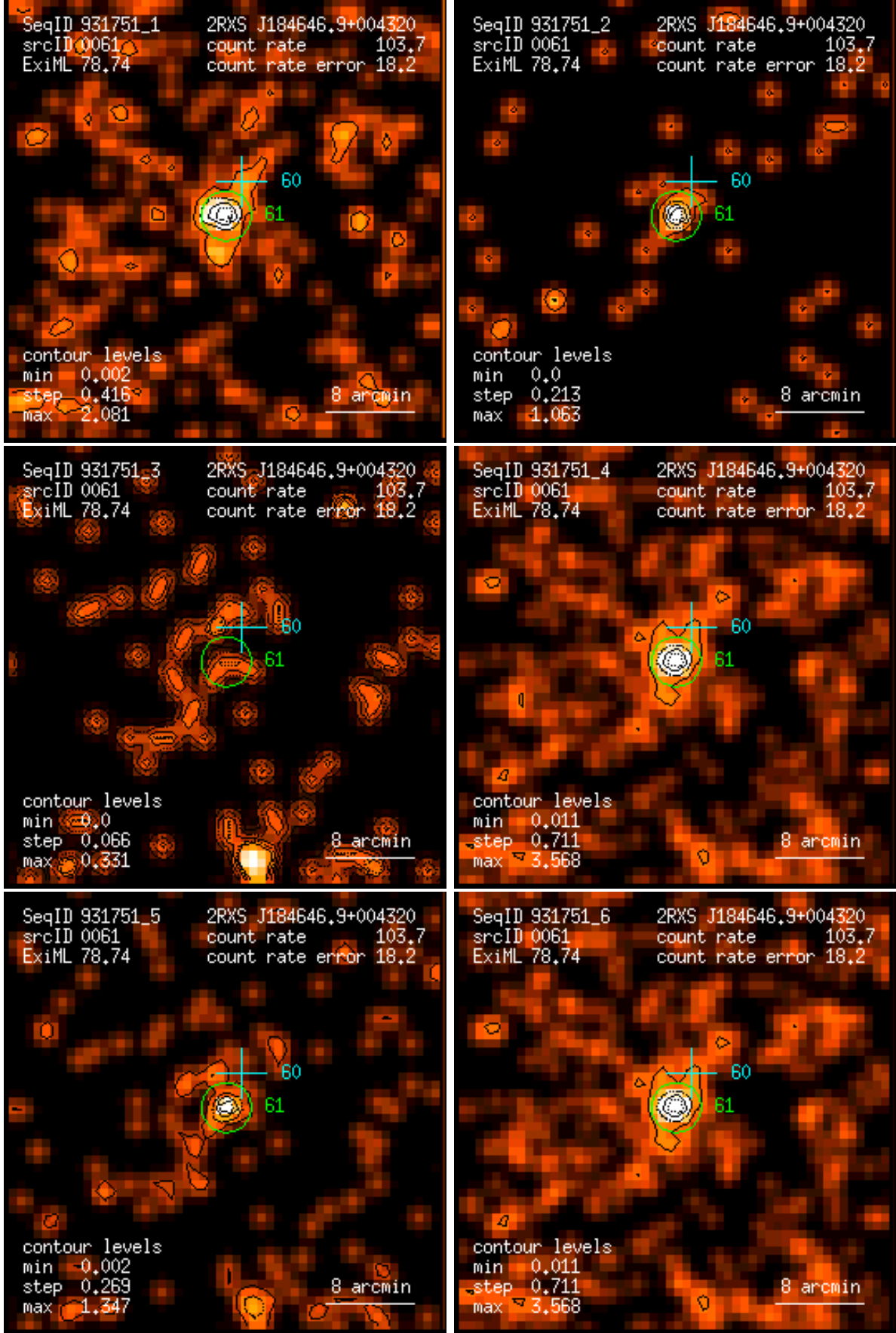
Figure 61: RASS 931751: detection 0061: band rate images, Gaussian filter: (1) PSPC channels 11 – 41, (2) 52 – 90, (3) 91 – 201, (4) 11 – 235, (5) 52 – 201, (6) 11 – 201. Broad band rates in counts/ks. Band rate contour levels in counts/ks/arcmin 2 .
