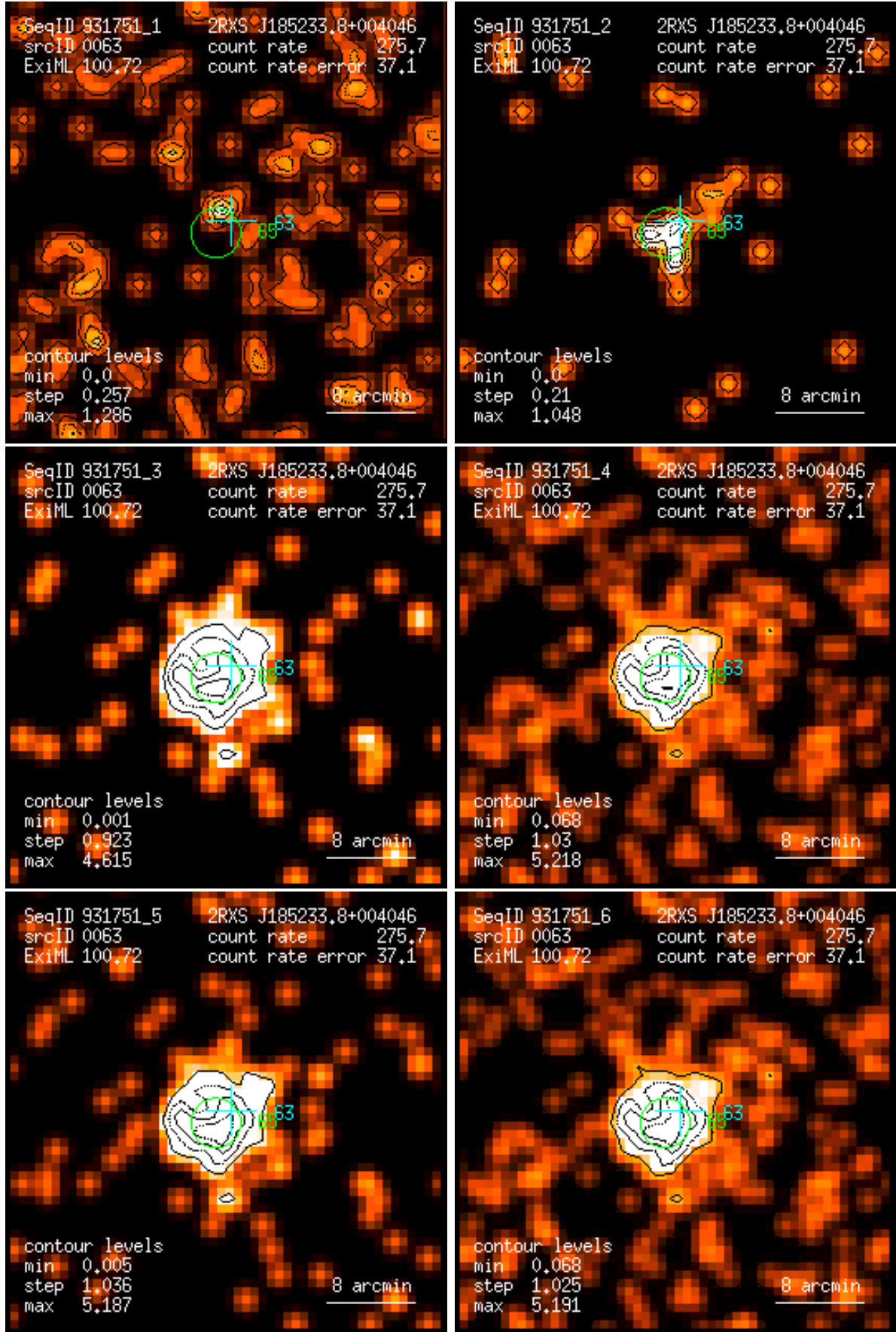
Figure 63: RASS 931751: detection 0063: band rate images, Gaussian filter: (1) PSPC channels 11 – 41, (2) 52 – 90, (3) 91 – 201, (4) 11 – 235, (5) 52 – 201, (6) 11 – 201. Broad band rates in counts/ks. Band rate contour levels in counts/ks/arcmin 2 .
