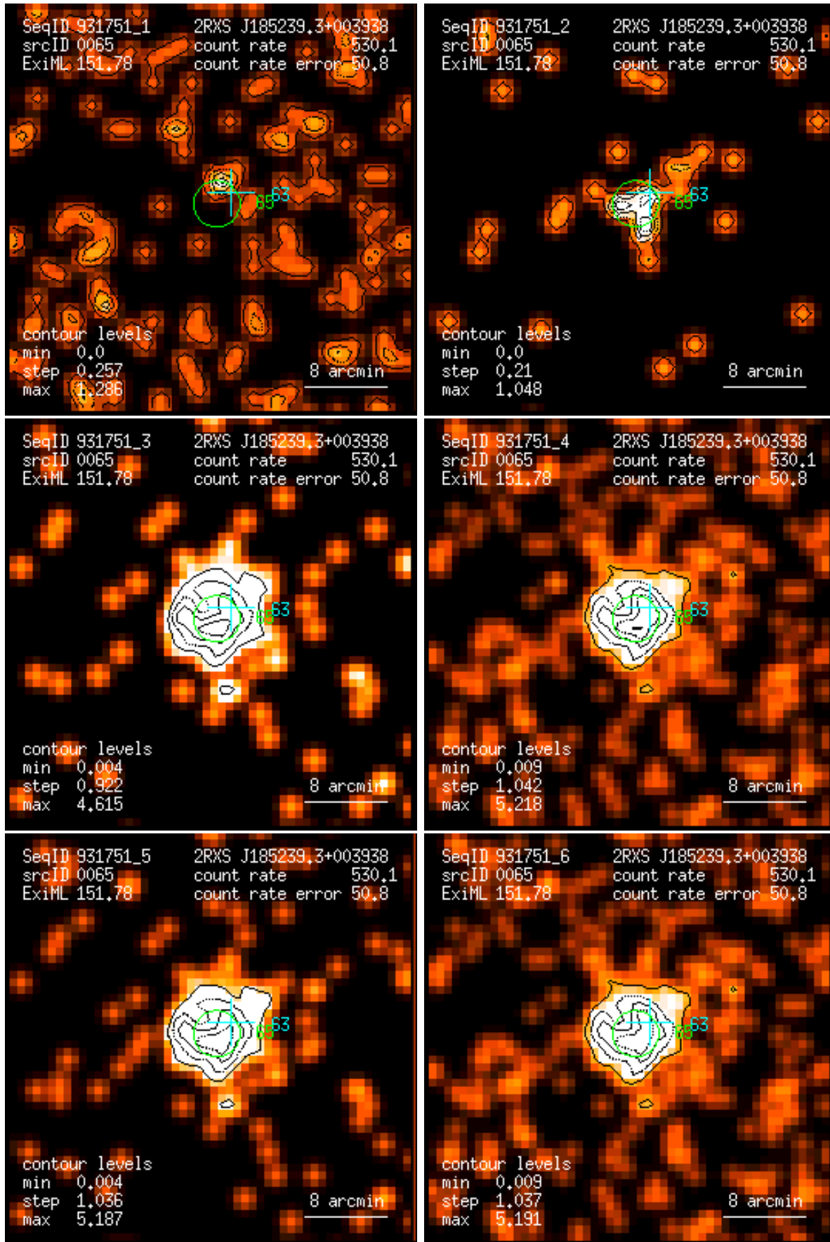
Figure 65: RASS 931751: detection 0065: band rate images, Gaussian filter: (1) PSPC channels 11 – 41, (2) 52 – 90, (3) 91 – 201, (4) 11 – 235, (5) 52 – 201, (6) 11 – 201. Broad band rates in counts/ks. Band rate contour levels in counts/ks/arcmin 2 .
