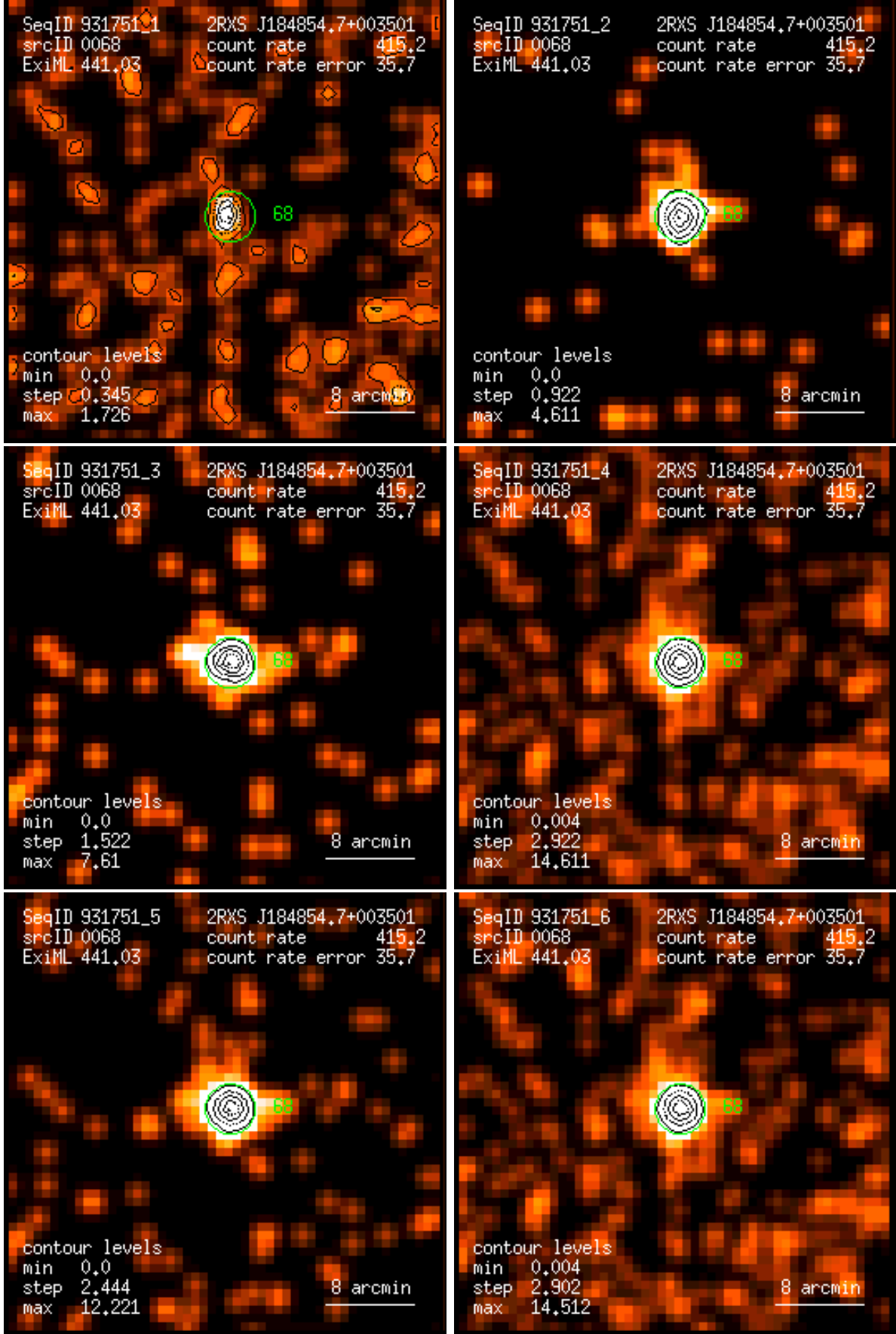
Figure 68: RASS 931751: detection 0068: band rate images, Gaussian filter: (1) PSPC channels 11 – 41, (2) 52 – 90, (3) 91 – 201, (4) 11 – 235, (5) 52 – 201, (6) 11 – 201. Broad band rates in counts/ks. Band rate contour levels in counts/ks/arcmin 2 .
