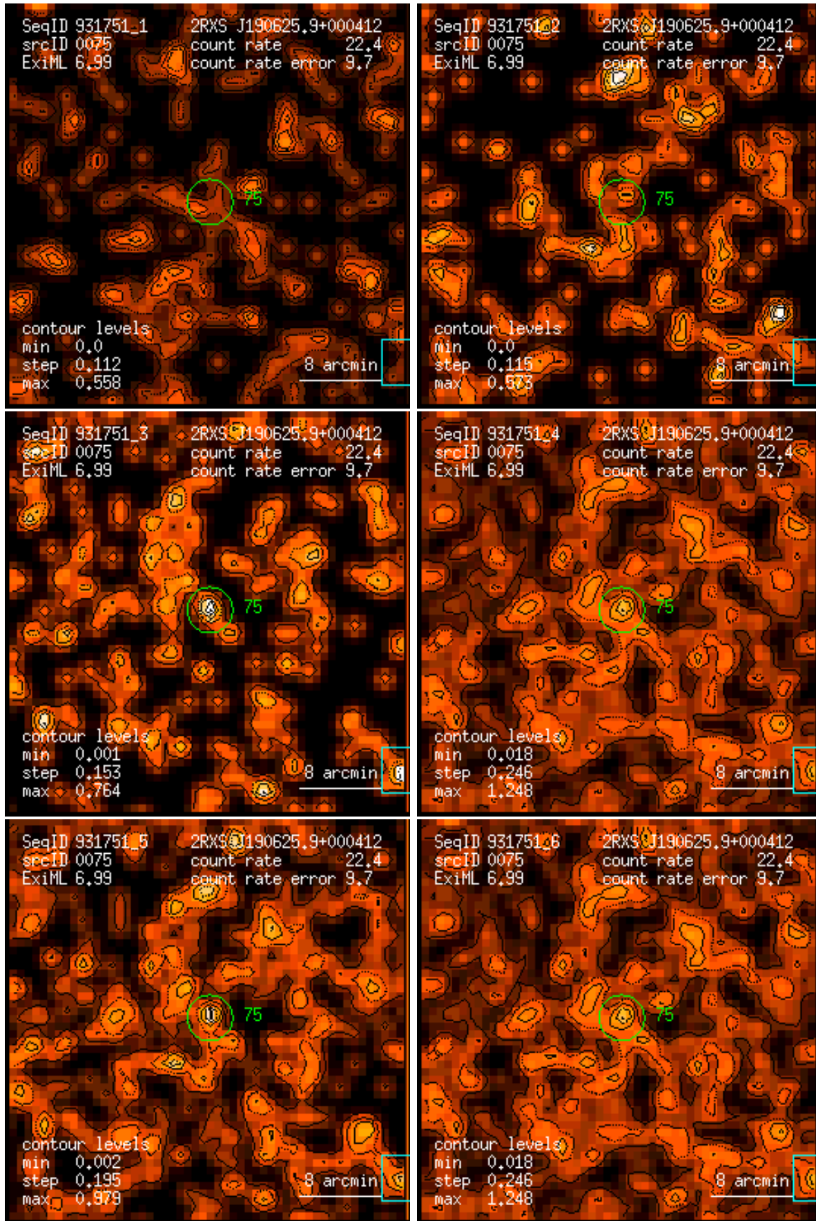
Figure 75: RASS 931751: detection 0075: band rate images, Gaussian filter: (1) PSPC channels 11 – 41, (2) 52 – 90, (3) 91 – 201, (4) 11 – 235, (5) 52 – 201, (6) 11 – 201. Broad band rates in counts/ks. Band rate contour levels in counts/ks/arcmin 2 .
