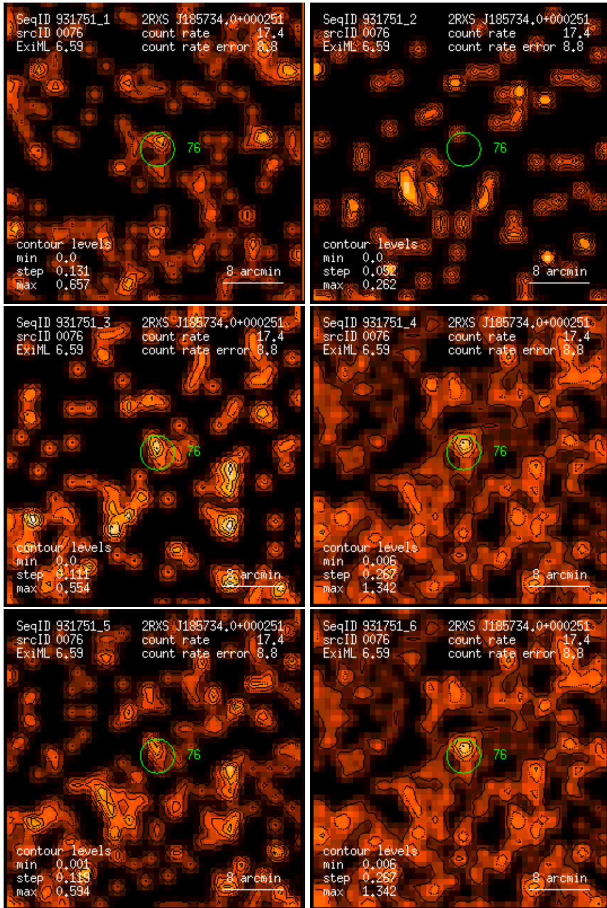
Figure 76: RASS 931751: detection 0076: band rate images, Gaussian filter: (1) PSPC channels 11 – 41, (2) 52 – 90, (3) 91 – 201, (4) 11 – 235, (5) 52 – 201, (6) 11 – 201. Broad band rates in counts/ks. Band rate contour levels in counts/ks/arcmin 2 .
