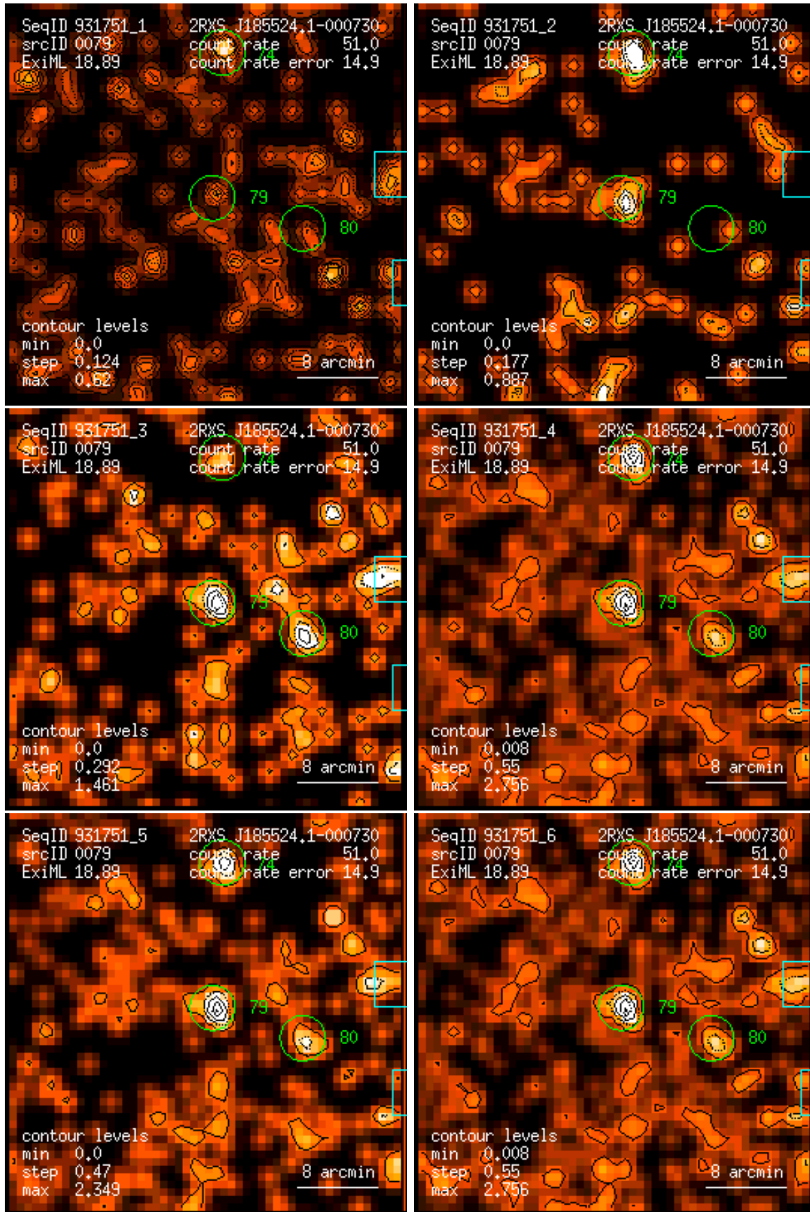
Figure 79: RASS 931751: detection 0079: band rate images, Gaussian filter: (1) PSPC channels 11 – 41, (2) 52 – 90, (3) 91 – 201, (4) 11 – 235, (5) 52 – 201, (6) 11 – 201. Broad band rates in counts/ks. Band rate contour levels in counts/ks/arcmin 2 .
